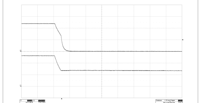
Shut-down enabled by disconnecting V_1 at: T_{P1} = +25^{\circ}\text{C} , V_1 = 53\text{ V} , I_o = 54.2\text{ A} resistive load.
