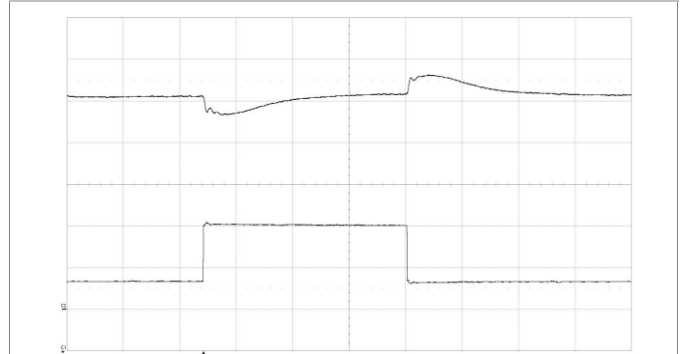
Output voltage response to load current step-change (13.5-40.7-13.5 A) at: T_{P1} = +25^{\circ}\text{C} , V_1 = 53\text{ V} .
