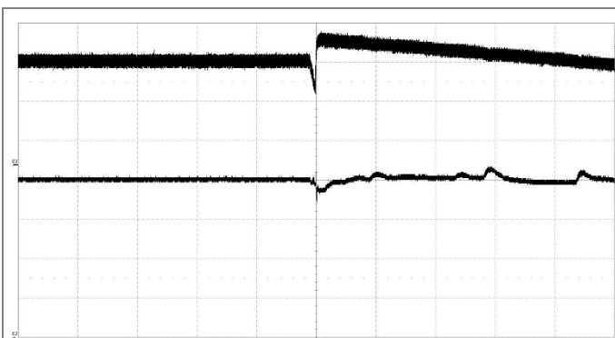
Output voltage response to input voltage transient at: T_{P1} = +25^{\circ}\text{C} , V_1 = 40\text{-}60\text{ V} , slew rate = 0.1V/ \mu\text{s} , I_o = 54\text{ A} , C_o = 1\text{ mF}
