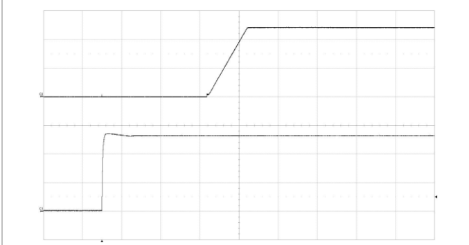
Start-up enabled by connecting V_1 at: T_{P1} = +25^{\circ}\text{C} , V_1 = 53\text{ V} , I_o = 54.2\text{ A} resistive load.
