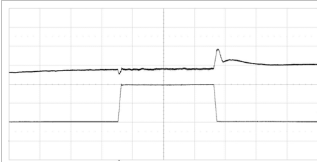
Output voltage response to load current Top trace: output voltage (100 mV/div.). Step-change (10-30-10 A) at: Bottom trace: load current (10 A/div.). T_{P1} = +25^\circ C , V_I = 12 V , V_O = 1.0 V Time scale: (0.1 ms/div.). di/dt = 2 A/\mu s , f_{sw} = 320 kHz C_O = 4000 \mu F
