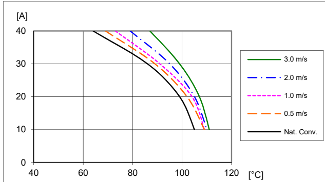
Output Current Derating, V_O = 0.6\text{ V}
