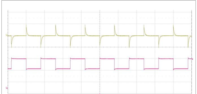
Output voltage response to load current step-change (1.39-2.09-1.39 A) at: T_{P1} = +25^\circ\text{C} , V_I = 110\text{ V} . Trace: output voltage (200 mV/div.). Bottom trace: load current (1 A/div.). Time scale: (1 ms/div.).
