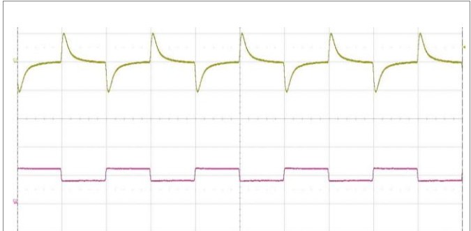
Output voltage response to load current step- change (4.15-6.225-4.15 A) at: T_{P1} = +25^{\circ}\text{C} , V_I = 110\text{ V} . Trace: output voltage (500 mV/div.). Bottom trace: load current (5 A/div.). Time scale: (1ms/div.).
