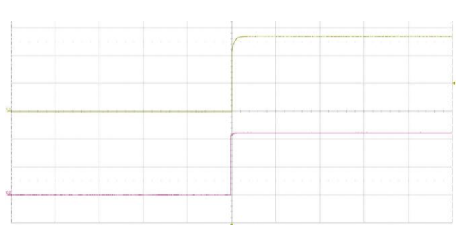
Start-up enabled by connecting V_I at: T_{P1} = +25^\circ\text{C} , V_I = 110\text{ V} , I_O = 2.78\text{ A} resistive load. Top trace: output voltage (20 V/div.). Bottom trace: input voltage (50 V/div.). Time scale: (50 ms/div.).
