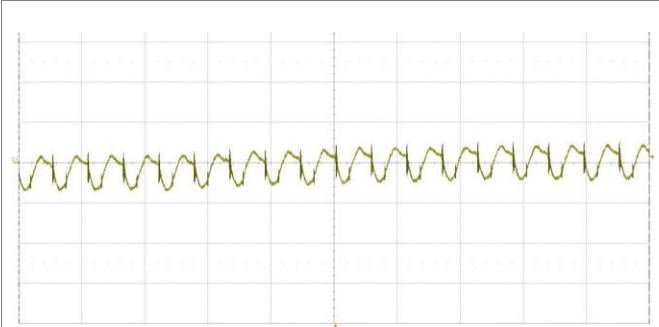
Output voltage ripple at: T_{P1} = +25^\circ\text{C} , V_i = 110\text{ V} , I_o = 4.16\text{ A} resistive load. Trace: output voltage (20 mV/div.). Time scale: (5 μs/div.).
