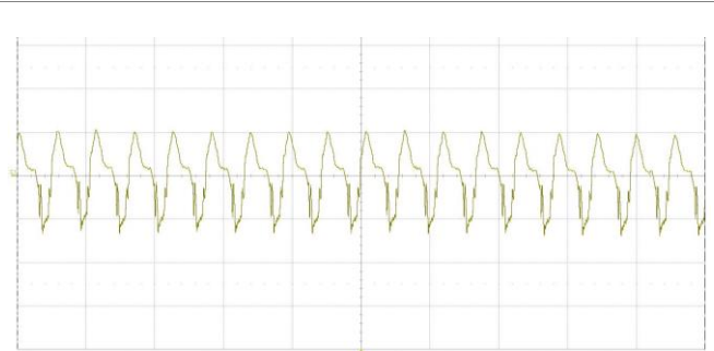
Output voltage ripple at: T_{P1} = +25^\circ\text{C} , V_I = 110\text{ V} , I_O = 2.78\text{ A} resistive load. Trace: output voltage (100 mV/div.). Time scale: (5 \mu\text{s} /div.).
