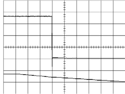
Shut-down enabled by disconnecting V_i at: T_{ref} = +25^\circ\text{C} , I_O = 18\text{ A} resistive load, V_i = 12.0\text{ V} . Top trace: output voltage (0.5 V/div.). Bottom trace: input voltage (10 V/div.). Time scale: 5.0 ms/div.
