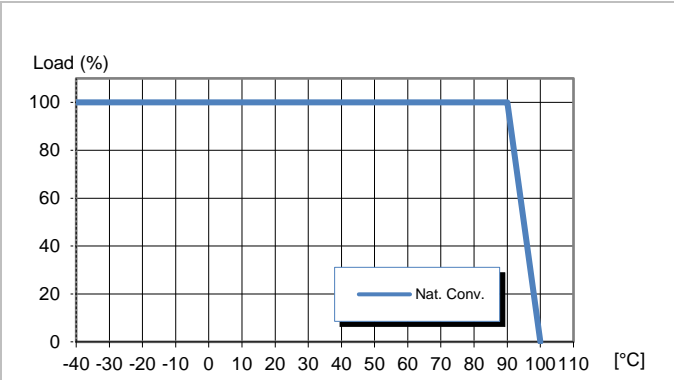
Available load vs. ambient air temperature. See Thermal Consideration section.
