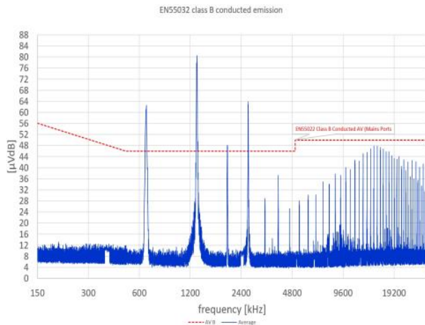
Without EMC filter, V_{in} = 54 V, max P_{out\_TDP}
