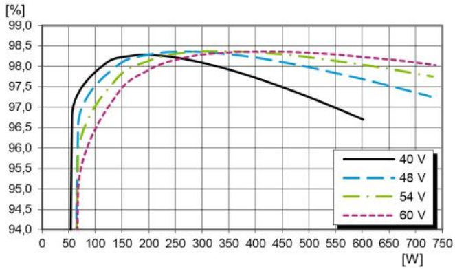
Efficiency vs. output power and input voltage at T_{PI} = +25^\circ
