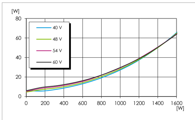
Dissipated power vs. output power and input voltage at T_{PI} = +90^{\circ}\text{C} . Above 1600W only peak t \leq 0.5\text{s}
