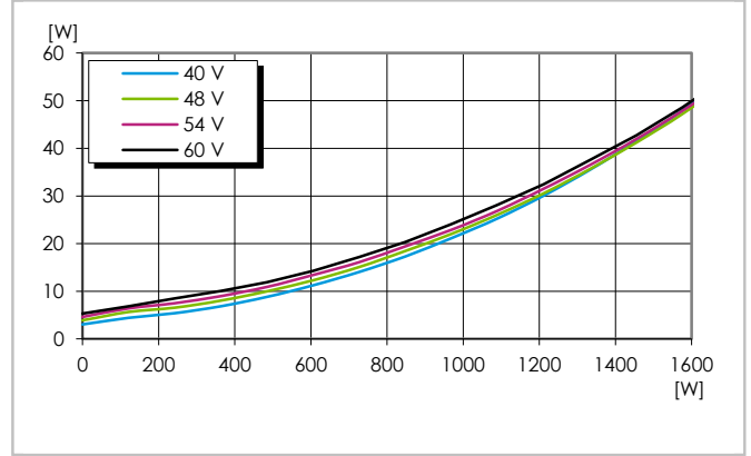
Dissipated power vs. output power at T_{P1} = +25^{\circ}\text{C}
