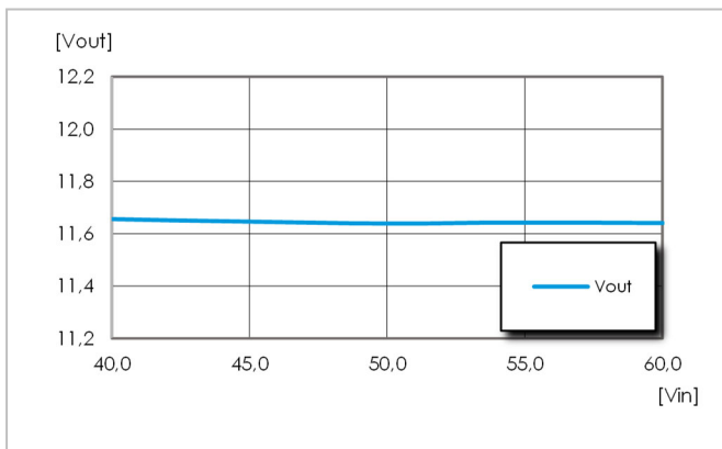
Output voltage vs. input voltage at T_{P1} = +90^{\circ}\text{C} , 100% of max P_{out\_TDP}
