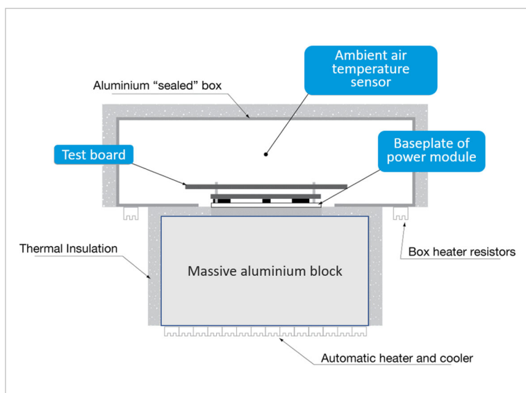
Picture: cold wall test set-up
