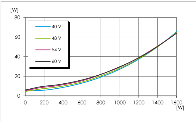
Dissipated power vs. output power and input voltage at T_{P1} = +90^{\circ}\text{C} . Above 1600W only peak t \leq 0,5\text{s}
