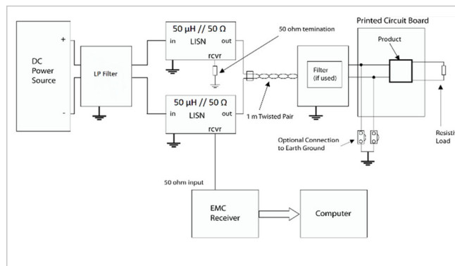
Test set-up
