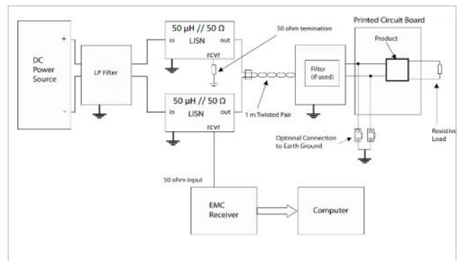
Test set-up
