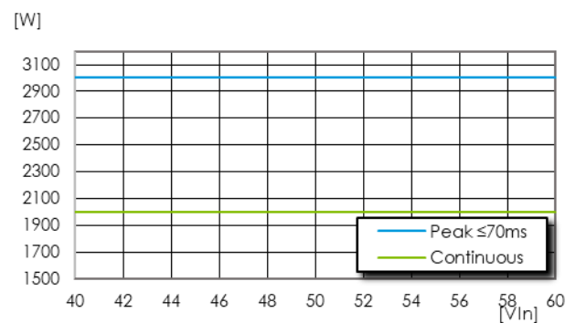
Available output power vs. input voltage, T_{PI} = +90^\circ C
