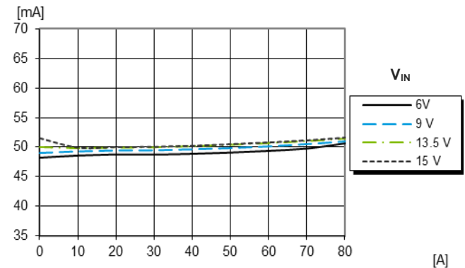
VCC=5V, Fs=550KHz
