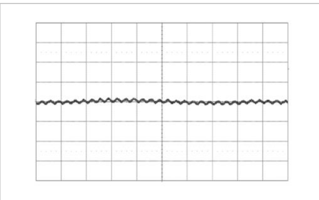
V_{in} = 13.5 V , I_{out} = 80 A , Scale: 5 mV/div, 1.5 μs/div, 20 MHz BW. C_{OUT} = 10 \times 470 \mu F/3 m\Omega POSCAP + 365 \times 10 μF ceramic.
