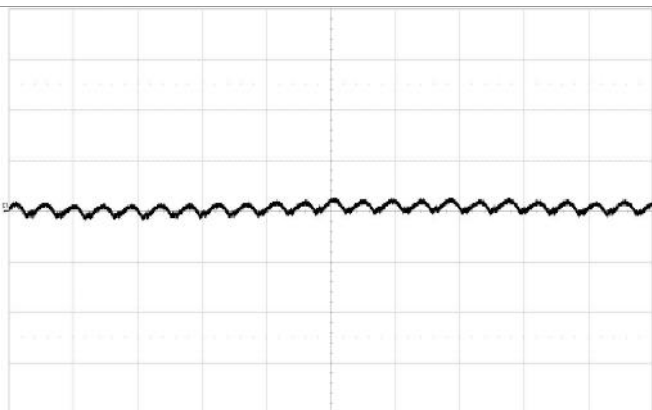
V_{in} = 13.5 V , I_o = 80 A , Scale: 5 mV/div, 1.5 \mu s /div, 20 MHz BW. C_{out} = 10 \times 470 \mu F / 3 m\Omega POSCAP + 365 \times 10 \mu F ceramic.
