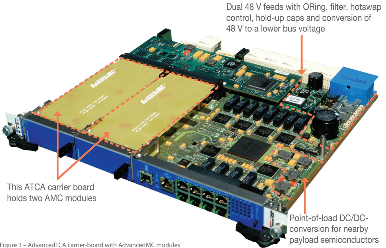
Figure 3 – AdvancedTCA carrier-board with AdvancedMC modules
