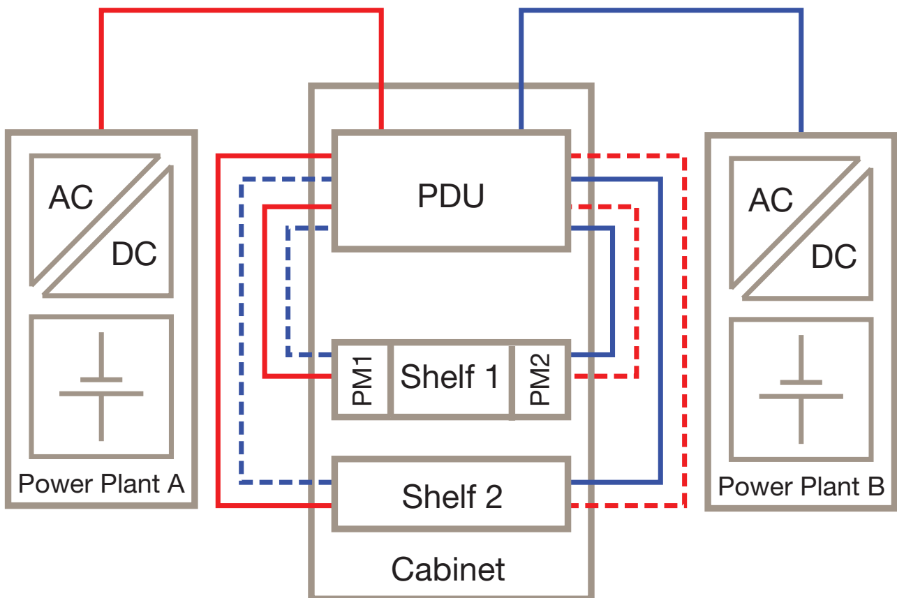
Figure 17 – Dual power feed general set-up
