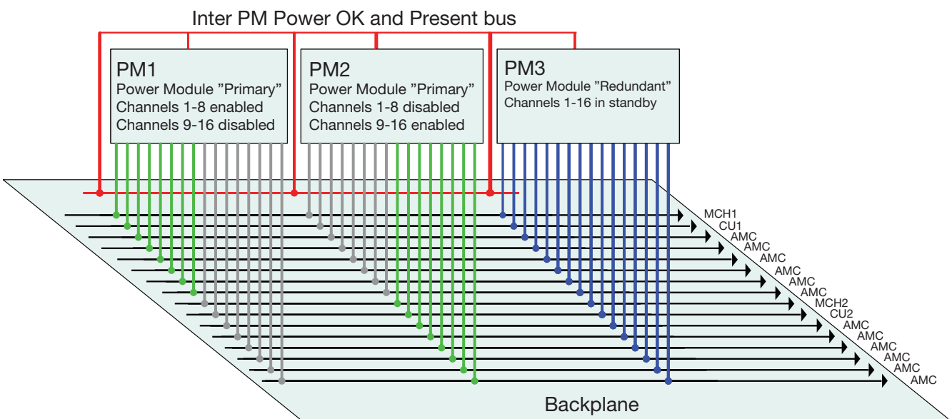
Figure 12 – Example of 2+1 redundant MicroTCA power module implementation
