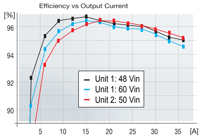
Figure 11 – PKM4304B PI and Efficiency dependent of input voltage
