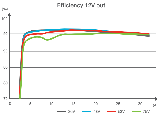
Figure 5 - BMR453 efficiency and voltage regulation illustrating the flat curve through the range of operation
