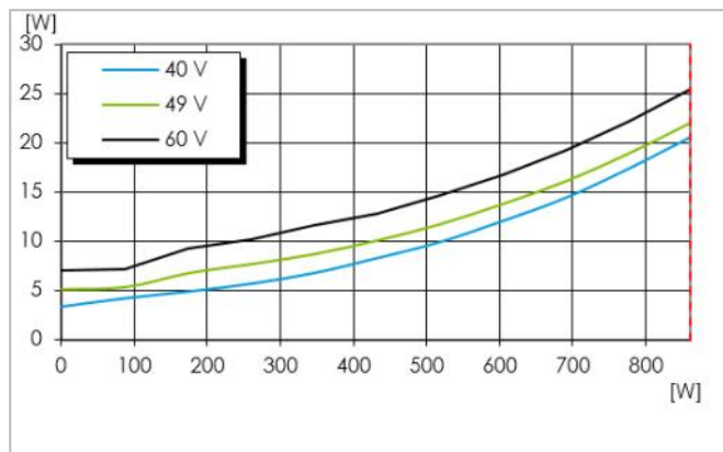
Dissipated power vs. load power at T_{P1} = +25^{\circ}C
