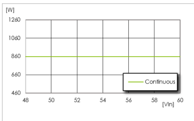
Available output power vs. input voltage, T_{P1} = +90^{\circ}C
