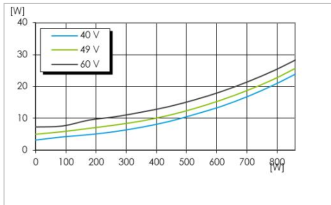
Dissipated power vs. output power and input voltage at T_{P1} = +90^{\circ}C
