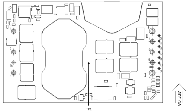
Open frame(Top view)
