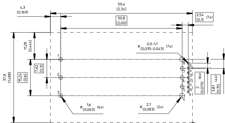
RECOMMENDED FOOTPRINT - TOP VIEW
