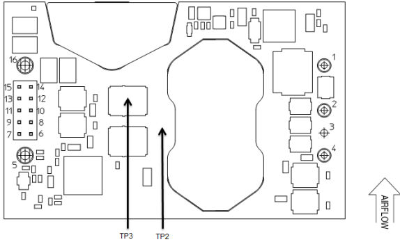
Base plate (Bottom view)
