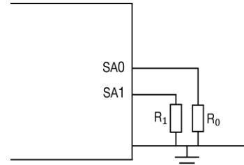
Schematic of connection of address resistors
