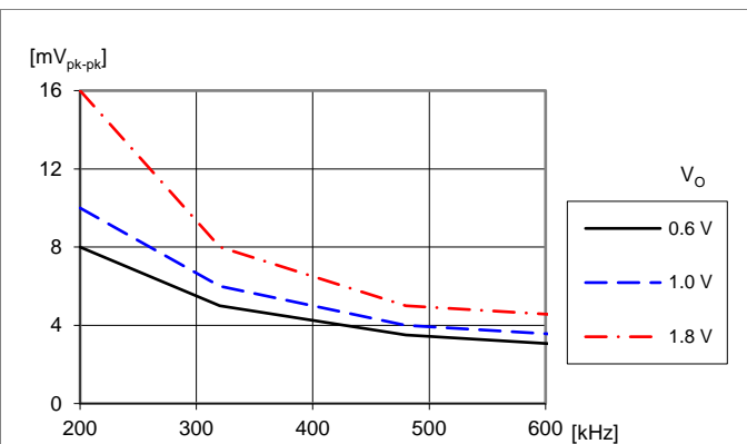
Output voltage ripple V_{pk-pk} vs. switching frequency at V_I = 12\text{ V} , I_O = \text{max } I_O , C_{OUT} = 3 \times 470\text{ }\mu\text{F}/4.5\text{ m}\Omega + 10 \times 100\text{ }\mu\text{F} . Frequency changed by PMBus command FREQUENCY_SWITCH.
