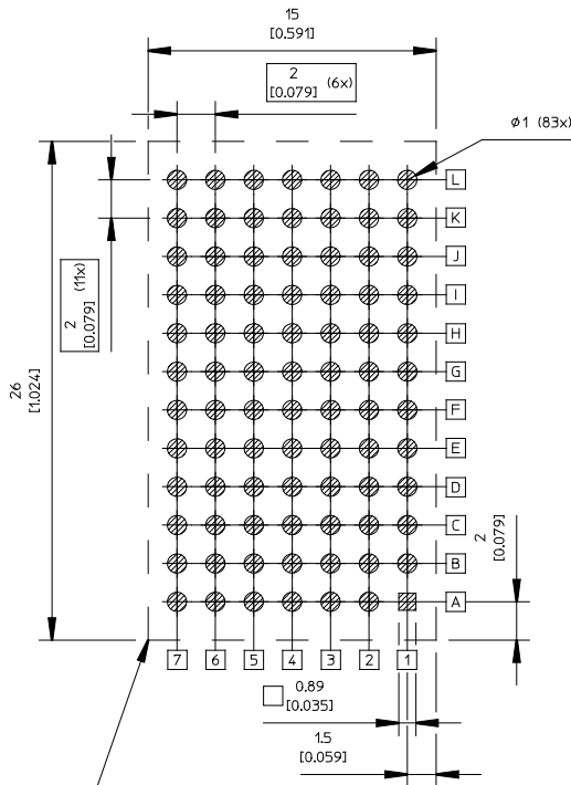
Recommended keep out area for user components
