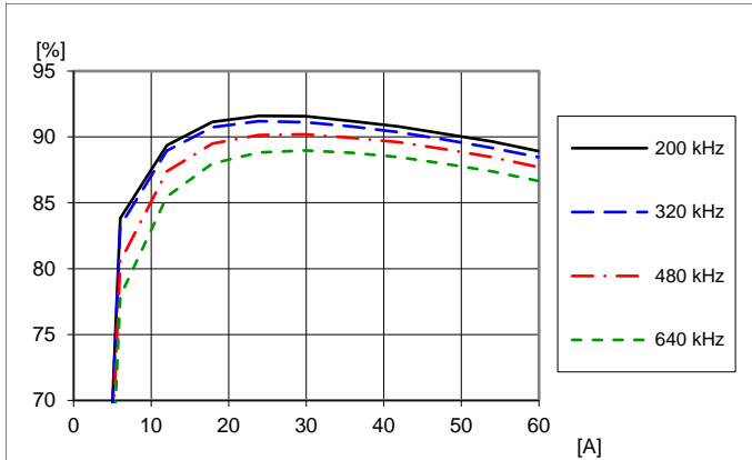
Efficiency vs. load current and switching frequency at V_I = 12\text{ V} , V_O = 1.0\text{ V} , C_{OUT} = 3 \times 470\text{ }\mu\text{F}/4.5\text{ m}\Omega + 10 \times 100\text{ }\mu\text{F} . Frequency changed by PMBus command FREQUENCY_SWITCH.
