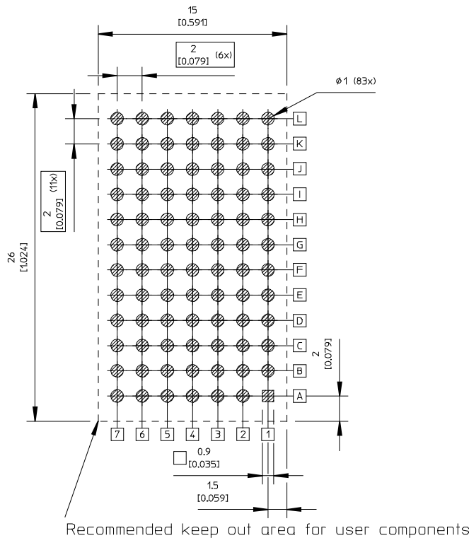
RECOMMENDED FOOTPRINT - TOP VIEW
