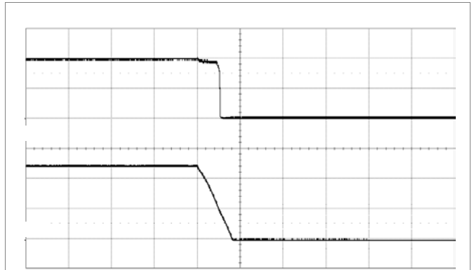
Shut-down enabled by disconnecting V_I at: T_{P1} = +25\text{ }^{\circ}\text{C} , V_I = 12\text{ V} , V_O = 1.0\text{ V} C_O = 470\text{ }\mu\text{F}/10\text{ m}\Omega , I_O = 40\text{ A} Top trace: output voltage (0.5 V/div.). Bottom trace: input voltage (5 V/div.). Time scale: (2 ms/div.).
