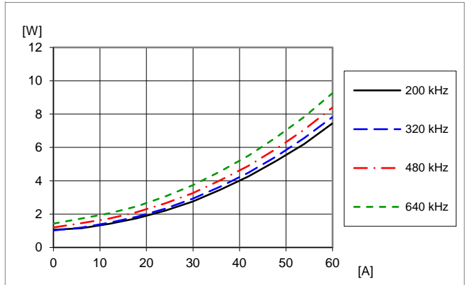
Dissipated power vs. load current and switching frequency at V_I = 12\text{ V} , V_O = 1.0\text{ V} , C_{OUT} = 3 \times 470\text{ }\mu\text{F}/4.5\text{ m}\Omega + 10 \times 100\text{ }\mu\text{F} . Frequency changed by PMBus command FREQUENCY_SWITCH.
