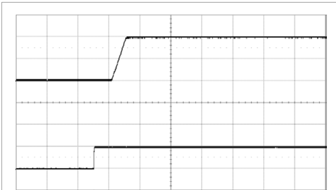
Start-up by enabling CTRL signal at: T_{P1} = +25\text{ }^{\circ}\text{C} , V_I = 12\text{ V} , V_O = 1.0\text{ V} C_O = 470\text{ }\mu\text{F}/10\text{ m}\Omega , I_O = 40\text{ A} Top trace: output voltage (0.5 V/div.). Bottom trace: CTRL signal (5 V/div.). Time scale: (20 ms/div.).
