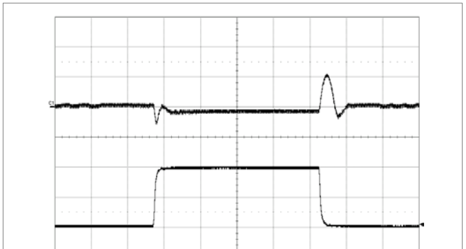
Output voltage response to load current step change (10–30–10 A), di/dt = 2\text{ A}/\mu\text{s} , at V_I = 12\text{ V} , C_{OUT} = 470\text{ }\mu\text{F}/10\text{ m}\Omega Compensation settings by product /001. Scale: 200 mV/div, 10 A/div, 100 \mu\text{s} /div.
