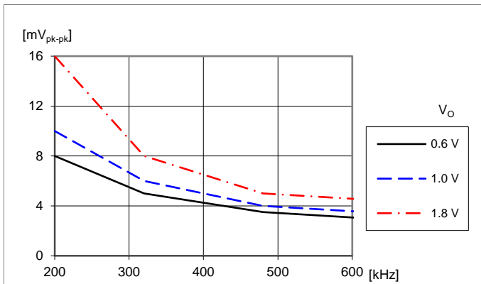
Output voltage ripple V_{pk-pk} vs. switching frequency at V_I = 12\text{ V} , I_O = \text{max } I_O , C_{OUT} = 3 \times 470\text{ }\mu\text{F}/4.5\text{ m}\Omega + 10 \times 100\text{ }\mu\text{F} . Frequency changed by PMBus command FREQUENCY_SWITCH.
