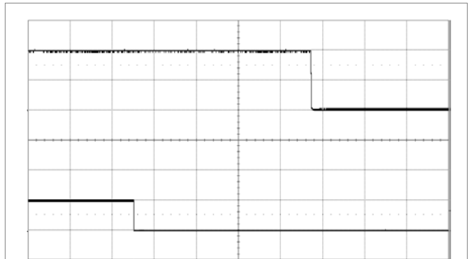
Shut-down enabled by disconnecting V_I at: T_{P1} = +25\text{ }^{\circ}\text{C} , V_I = 12\text{ V} , V_O = 1.0\text{ V} C_O = 470\text{ }\mu\text{F}/10\text{ m}\Omega , I_O = 40\text{ A} Top trace: output voltage (0.5 V/div.). Bottom trace: CTRL signal (5 V/div.). Time scale: (2 ms/div.).
