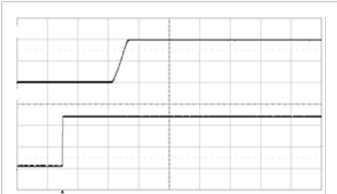
Start-up enabled by connecting V_I at: T_{P1} = +25\text{ }^{\circ}\text{C} , V_I = 12\text{ V} , V_O = 1.0\text{ V} C_O = 470\text{ }\mu\text{F}/10\text{ m}\Omega , I_O = 40\text{ A} Top trace: output voltage (0.5 V/div.). Bottom trace: input voltage (5 V/div.). Time scale: (20 ms/div.).
