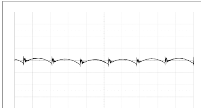
Fundamental output voltage ripple at V_I = 12\text{ V} , I_o = 60\text{ A} , C_{OUT} = 3 \times 470\text{ }\mu\text{F}/4.5\text{ m}\Omega + 10 \times 100\text{ }\mu\text{F} Scale: 5 mV/div, 2 \mu\text{s} /div, 20 MHz bandwidth. See section Output Ripple and Noise.
