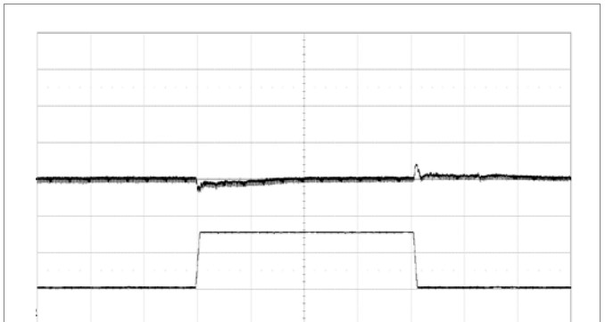
Output voltage response to load current step change (15–45–15 A), di/dt = 2\text{ A}/\mu\text{s} , at V_I = 12\text{ V} , C_{OUT} = 6 \times 470\text{ }\mu\text{F}/4.5\text{ m}\Omega + 10 \times 100\text{ }\mu\text{F} . Compensation settings by default PID and optimized NLR. Scale: 50 mV/div, 20 A/div, 200 \mu\text{s} /div.
