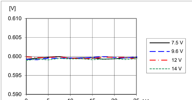
Output voltage vs load current.
