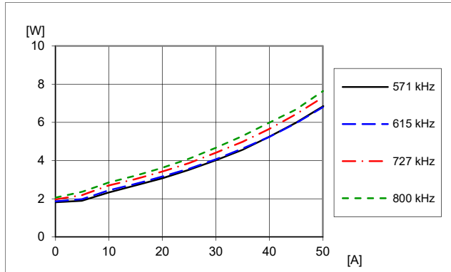
Dissipated power vs. load current and switching frequency at V_I = 12\text{ V} , V_O = 1.0\text{ V} , C_O = 4 \times 330\text{ }\mu\text{F}/10\text{ m}\Omega + 12 \times 100\text{ }\mu\text{F} . Frequency changed by PMBus command FREQUENCY_SWITCH.
