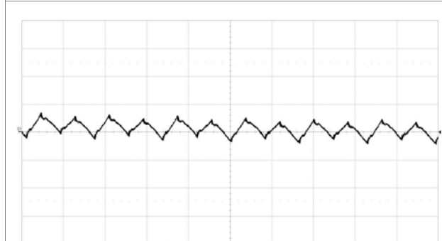
Fundamental output voltage ripple at V_I = 12\text{ V} , I_o = 34\text{ A} , C_{OUT} = 4 \times 330\text{ }\mu\text{F}/10\text{ m}\Omega + 12 \times 100\text{ }\mu\text{F} Scale: 5 mV/div, 1 \mu\text{s} /div, 20 MHz bandwidth. See section Output Ripple and Noise.
