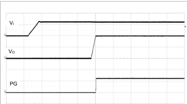
Output enabled by applying V_i . V_i = 12\text{ V} , I_o = 50\text{ A} . TON\_DELAY = TON\_RISE = 5\text{ ms} , POWER\_GOOD\_DELAY = 1\text{ ms} . USER\_CONFIG = 0x1084 (page0) / 0x10A4 (page1) (default). Scale from top: 10, 0.5, 2 V/div, 20 ms/div.
