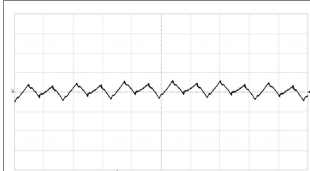
Fundamental output voltage ripple at V_i = 12\text{ V} , I_o = 28\text{ A} , C_{OUT} = 4 \times 330\text{ }\mu\text{F}/10\text{ m}\Omega + 12 \times 100\text{ }\mu\text{F} Scale: 5 mV/div, 1 \mu\text{s}/\text{div} , 20 MHz bandwidth. See section Output Ripple and Noise.
