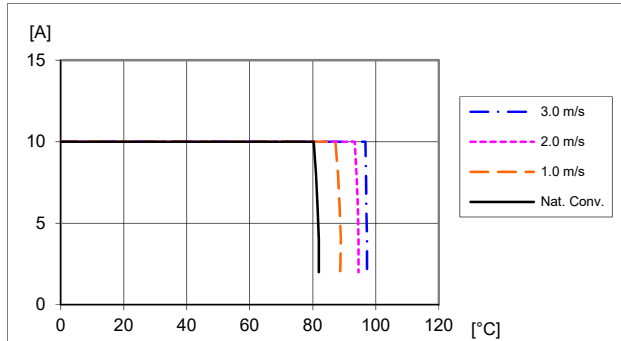
Available load current vs. ambient air temperature and airflow at V_i = 12\text{ V} . Another output is enabled with full load.
