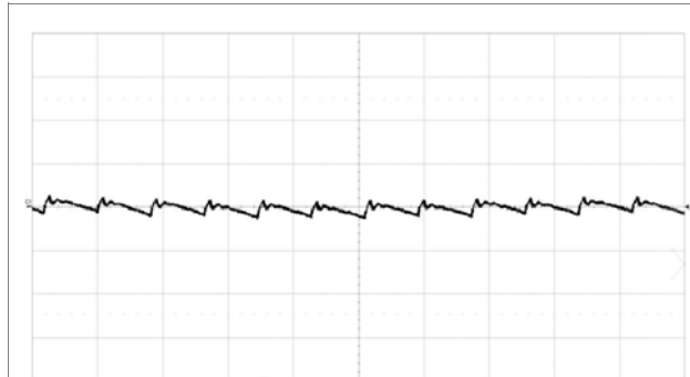
dFundamental output voltage ripple at V_I = 12\text{ V} , I_o = 50\text{ A} , C_{OUT} = 4 \times 330\text{ }\mu\text{F}/10\text{ m}\Omega + 12 \times 100\text{ }\mu\text{F} Scale: 5 mV/div, 1 \mu\text{s}/\text{div} , 20 MHz bandwidth. See section Output Ripple and Noise.
