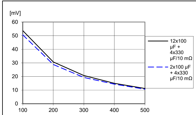
Load transient peak voltage deviation vs. ASCR gain and external capacitance. Step (12.5–37.5–12.5 A). V_I = 12\text{ V} , V_O = 1.0\text{ V} , f_{sw} = 615\text{ kHz} , ASCR residual = 90, di/dt = 2\text{ A}/\mu\text{s} . ASCR gain changed by PMBus command ASCR_CONFIG.
