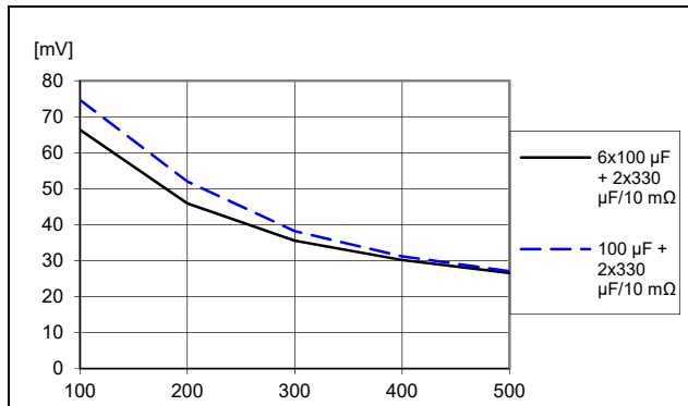
Load transient peak voltage deviation vs. ASCR gain and external capacitance. Step (6.25–18.75–6.25 A). V_I = 12\text{ V} , V_O = 1.0\text{ V} , f_{sw} = 615\text{ kHz} , ASCR residual = 90, di/dt = 2\text{ A}/\mu\text{s} . ASCR gain changed by PMBus command ASCR_CONFIG.
