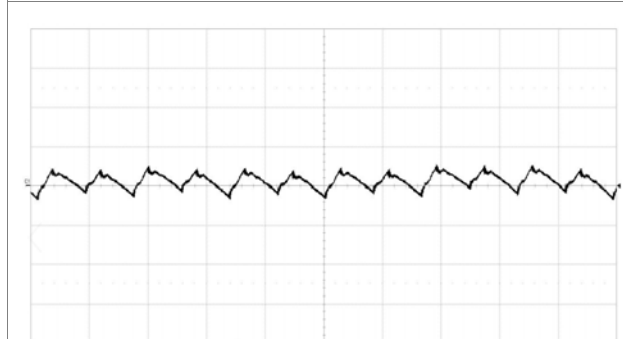
Fundamental output voltage ripple at V_i = 12\text{ V} , I_o = 45\text{ A} , C_{OUT} = 4 \times 330\text{ }\mu\text{F}/10\text{ m}\Omega + 12 \times 100\text{ }\mu\text{F} Scale: 5 mV/div, 1 \mu\text{s} /div, 20 MHz bandwidth. See section Output Ripple and Noise.
