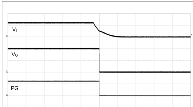
Output disabled by removing V_i . V_i = 12\text{ V} , I_o = 50\text{ A} . Scale from top: 10, 0.5, 2 V/div, 20 ms/div.
