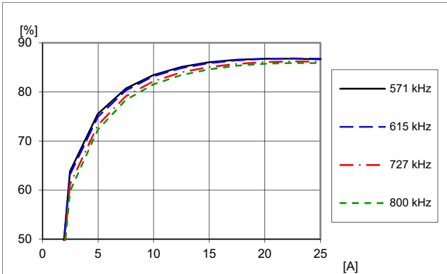
Efficiency vs. load current and switching frequency at V_I = 12\text{ V} , V_O = 1.0\text{ V} , C_O = 2 \times 330\text{ }\mu\text{F}/10\text{ m}\Omega + 6 \times 100\text{ }\mu\text{F} . Frequency changed by PMBus command FREQUENCY_SWITCH.
