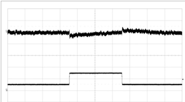
Output voltage response to load current step change (25%–75%–25%) at V_i = 12\text{ V} , C_{OUT} = 2 \times 330\text{ }\mu\text{F}/10\text{ m}\Omega + 6 \times 100\text{ }\mu\text{F} , di/dt = 2\text{ A}/\mu\text{s} , ACSR Gian=200 and ASCR Residual=90. Scale from top: 50 mV/div, 5 A/div, 200us/div. Note: Sense pins are connected to load.
