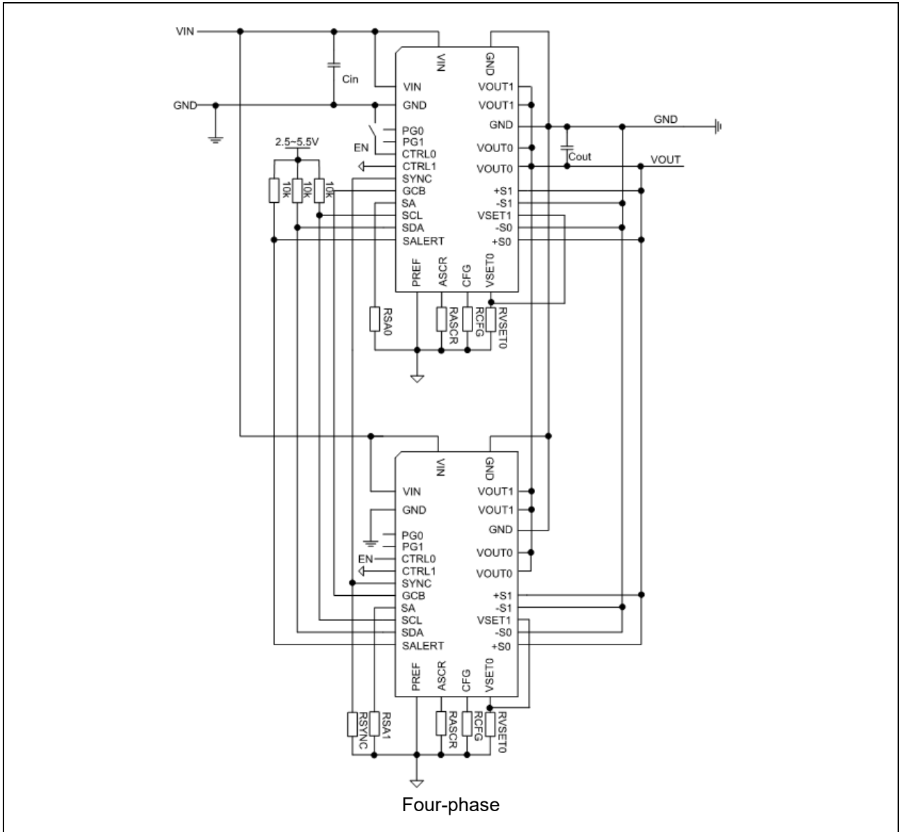
Parallel operation.
