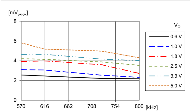
Output voltage ripple V_{pk-pk} vs. switching frequency at V_I = 12\text{ V} , I_O = \text{max } I_O , C_O = 2 \times 330\text{ }\mu\text{F}/10\text{ m}\Omega + 6 \times 100\text{ }\mu\text{F} . Frequency changed by PMBus command FREQUENCY_SWITCH.
