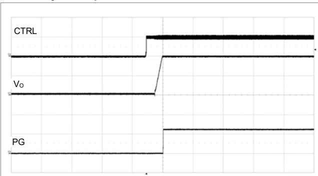
Output enabled by CTRL pin. V_i = 12\text{ V} , I_o = 50\text{ A} . TON\_DELAY = TON\_RISE = 5\text{ ms} , POWER\_GOOD\_DELAY = 1\text{ ms} . Scale from top: 10, 0.5, 2 V/div, 20 ms/div.
