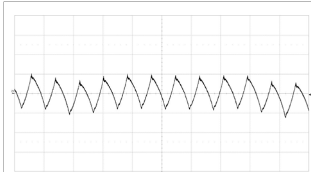
Fundamental output voltage ripple at V_i = 12\text{ V} , I_o = 10\text{ A} , C_{OUT} = 2 \times 330\text{ }\mu\text{F}/10\text{ m}\Omega + 6 \times 100\text{ }\mu\text{F} Scale: 10 mV/div, 2 \mu\text{s} /div, 20 MHz bandwidth. See section Output Ripple and Noise.
