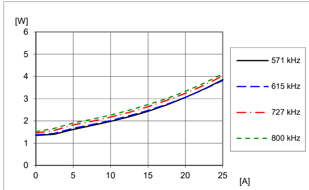
Dissipated power vs. load current and switching frequency at V_I = 12\text{ V} , V_O = 1.0\text{ V} , C_O = 2 \times 330\text{ }\mu\text{F}/10\text{ m}\Omega + 6 \times 100\text{ }\mu\text{F} . Frequency changed by PMBus command FREQUENCY_SWITCH.
