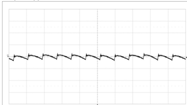
Fundamental output voltage ripple at V_i = 12 V , I_o = 25 A , C_{OUT} = 2 \times 330 \mu F / 10 m\Omega + 6 \times 100 \mu F Scale: 10 mV/div, 2 \mu s /div, 20 MHz bandwidth. See section Output Ripple and Noise.
