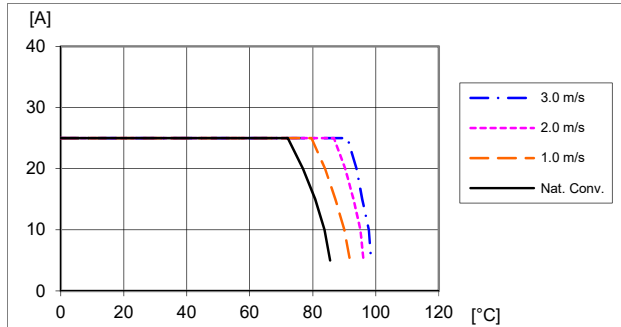
Available load current vs. ambient air temperature and airflow at V_i = 12 V . Another output is enabled with full load.
