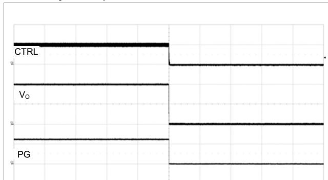
Output disabled by CTRL pin. V_i = 12\text{ V} , I_o = 50\text{ A} . Scale from top: 10, 0.5, 2 V/div, 20 ms/div.
