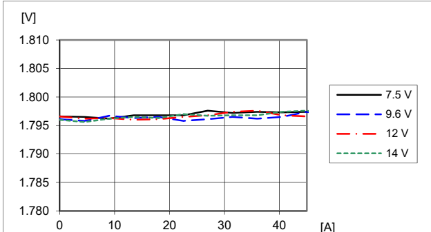
Output voltage vs load current.
