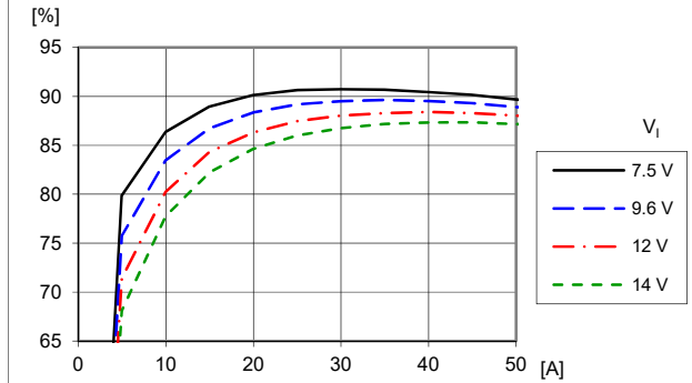
Efficiency vs. load current and input voltage.
