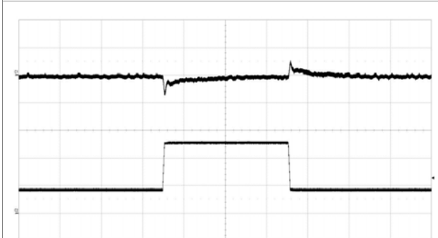
Output voltage response to load current step change (25%–75%–25%) at V_I = 12\text{ V} , C_{OUT} = 4 \times 330\text{ }\mu\text{F}/10\text{ m}\Omega + 12 \times 100\text{ }\mu\text{F} , di/dt = 2\text{ A}/\mu\text{s} , ACSR Gain=200 and ACSR Residual=90. Scale from top: 50 mV/div, 10 A/div, 200 \mu\text{s} /div. Note: Sense pins are connected to load.
