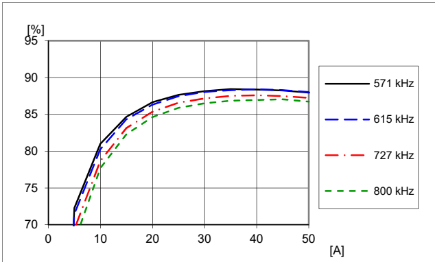
Efficiency vs. load current and switching frequency at V_I = 12\text{ V} , V_O = 1.0\text{ V} , C_O = 4 \times 330\text{ }\mu\text{F}/10\text{ m}\Omega + 12 \times 100\text{ }\mu\text{F} . Frequency changed by PMBus command FREQUENCY_SWITCH.
