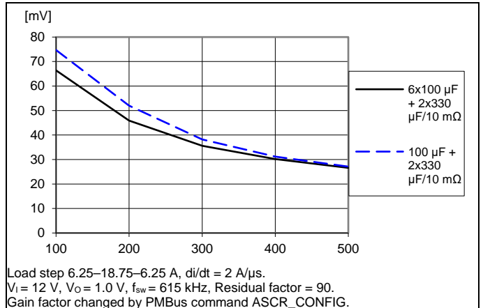
Voltage deviation vs. control loop gain setting and output capacitance.
