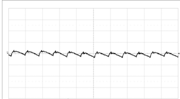
Fundamental output voltage ripple at V_I = 12\text{ V} , I_o = 50\text{ A} , C_{OUT} = 4 \times 330\text{ }\mu\text{F}/10\text{ m}\Omega + 12 \times 100\text{ }\mu\text{F} Scale: 5 mV/div, 1 \mu\text{s} /div, 20 MHz bandwidth. See section Output Ripple and Noise.
