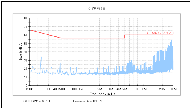
EMI with filter, EN55022 Test method and limits are the same as EN55022.
