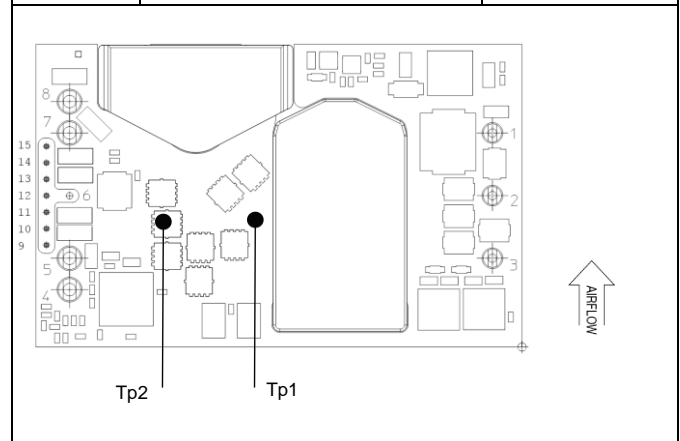
Base plate (Bottom view)
