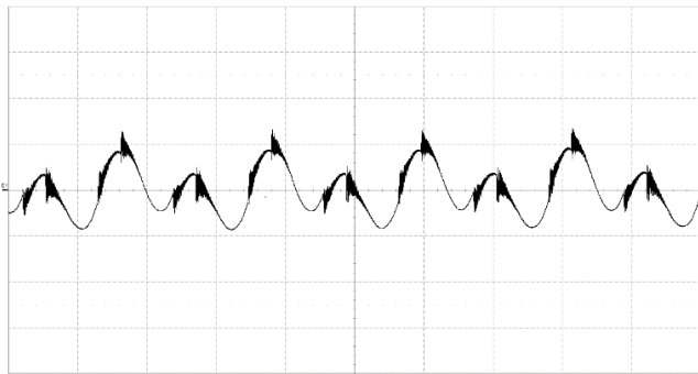
Output voltage ripple at: T_{P1} = +25^\circ\text{C} , V_i = 53\text{ V} , I_o = 75\text{ A} resistive load.
