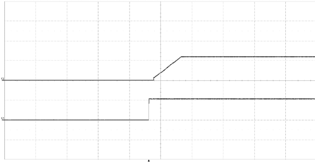
Start-up enabled by connecting V_i at: T_{P1} = +25^\circ\text{C} , V_i = 53\text{ V} , I_o = 75\text{ A} resistive load.
