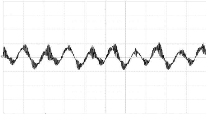
Output voltage ripple at: T_{P1} = +25^\circ\text{C} , V_i = 53\text{ V} , I_o = 220\text{ A} resistive load.
