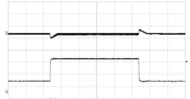
Output voltage response to load current step- change 18.75-56.25-18.75 A (2 A/ \mu\text{s} ) at: T_{P1} = +25^\circ\text{C} , V_i = 53\text{ V} .
