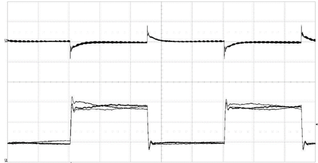
Output voltage response to load current step- change 56-168-56 A (2 A/ \mu\text{s} ) at: T_{P1} = +25^\circ\text{C} , V_i = 53\text{ V} .
