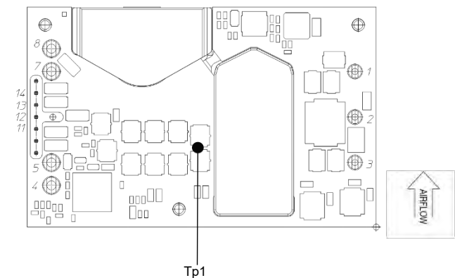
Base plate (Bottom view)
