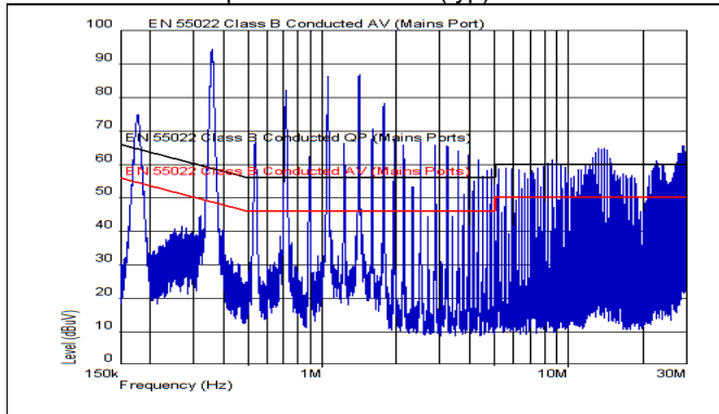
EMI without filter. EN55032 Test method and limits are the same as EN55022. 470 \mu F 100V input capacitor and 470 \mu F 16 V OS-CON output capacitor used.
