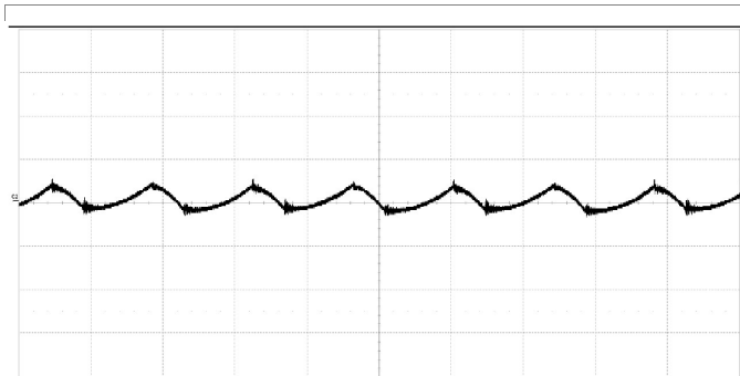
Output voltage ripple at: T_{PI} = +25^\circ\text{C} , V_i = 54\text{ V} , I_o = 110\text{ A} constant resistance. Trace: output voltage 100 mV/div. Time scale: 2 \mu\text{s} /div.
