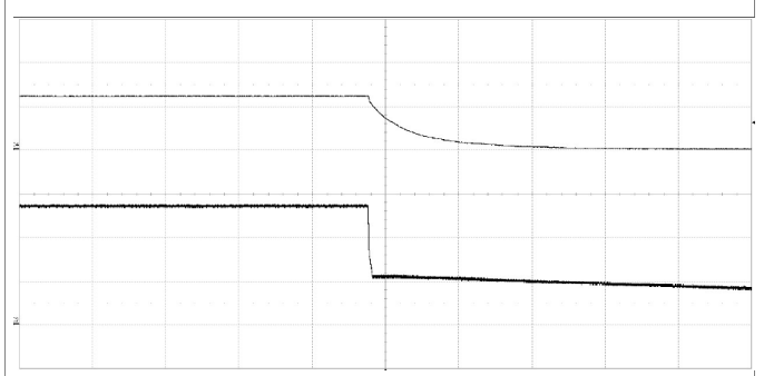
Shut-down enabled by disconnecting V_i at: T_{PI} = +25^\circ\text{C} , V_i = 54\text{ V} , I_o = 110\text{ A} resistive load. Top trace: output voltage 10 V/div. Bottom trace: input voltage 20V/div. Time scale: 5 ms/div.
