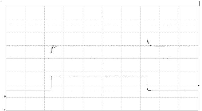
Output voltage response to load current step- change 27.5-82.5-27.5 A (2 A/ \mu\text{s} ) at: T_{PI} = +25^\circ\text{C} , V_i = 54\text{ V} . Top trace: output voltage 1 V/div. Bottom trace: load current 50 A/div. Time scale: 2 ms/div.
