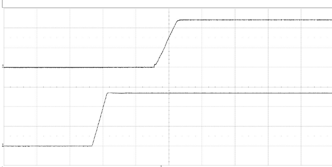
Start-up enabled by connecting V_i at: T_{PI} = +25^\circ\text{C} , V_i = 54\text{ V} , I_o = 110\text{ A} constant resistance. Top trace: output voltage 5 V/div. Bottom trace: input voltage 20 V/div. Time scale: 20 ms/div
