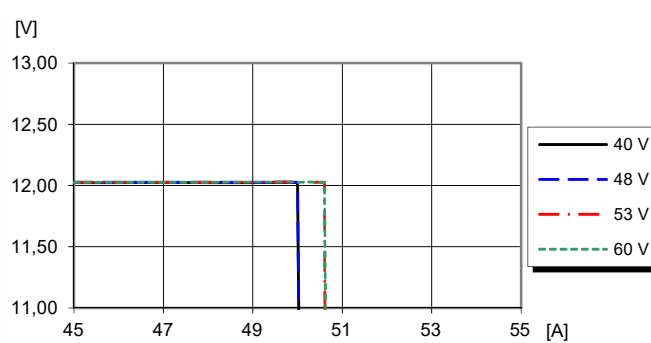
Output voltage vs. load current and input voltage at I_o > \text{max } I_o , T_{P1} = +25^{\circ}\text{C} .
