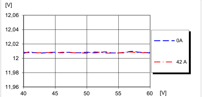
Output voltage vs. input voltage and load current at T_{P1} = +25^{\circ}\text{C} .
