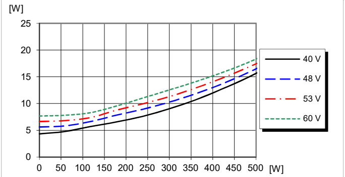
Dissipated power vs. output power and input voltage at T_{P1} = +25^{\circ}\text{C} .
