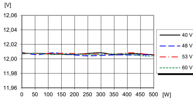
Output voltage vs. output power and input voltage at T_{P1} = +25^{\circ}\text{C} .
