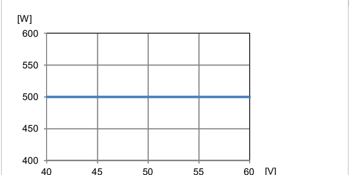
Output power vs. input voltage at T_{P1} = +25^{\circ}\text{C} .
