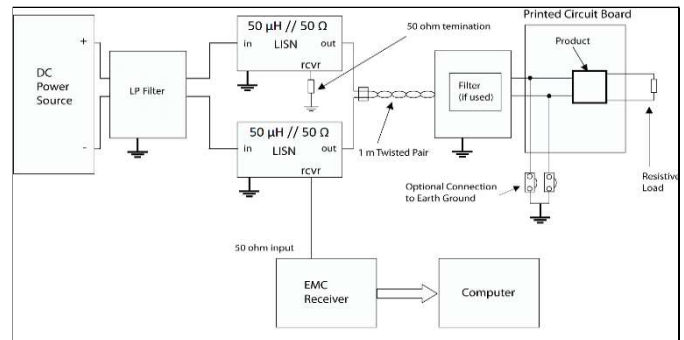
Test set-up
