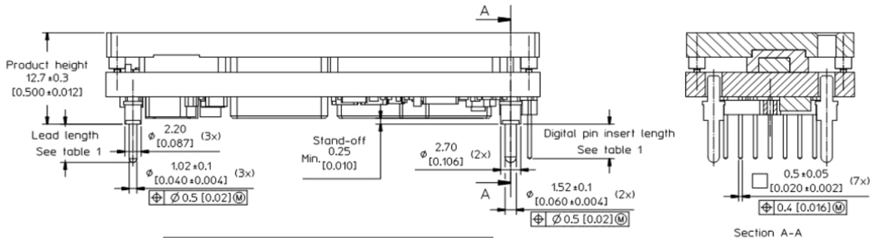
TOP VIEW Pin position according to recommended footprint
