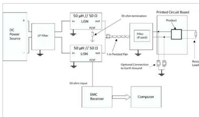
Test set-up
