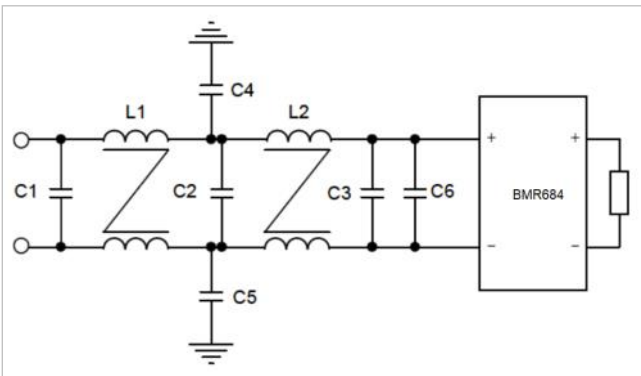
Filter components: C1, C2 = 4 x 4.7 µF MLCC; C3 = 3 x 4.7 µF MLCC; C4, C5 = 2 x 10nF 2kV MLCC; C6 = 470 µF; L1, L2 = 0.63mH (Pulse P0469NL)
