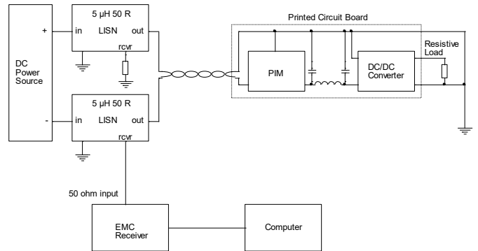
Test set-up
