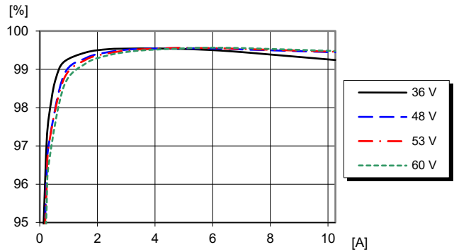
Efficiency vs. load current and input voltage at T_{P1} = +25\text{ }^{\circ}\text{C}
