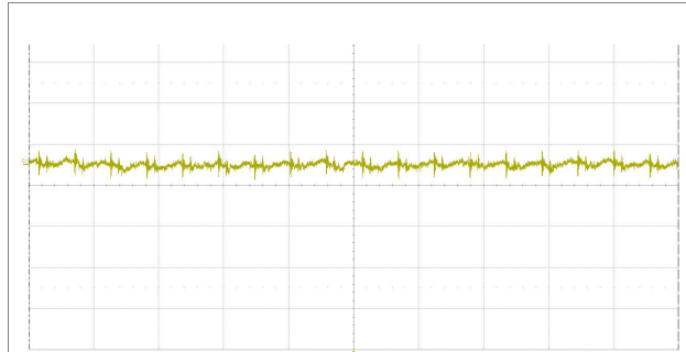
Output voltage ripple at: T_{P1} = +25^{\circ}\text{C} , V_I = 110\text{ V} , I_O = 6\text{ A} resistive load. Trace: output voltage (20 mV/div.). Time scale: (5 \mu\text{s} /div.). 20MHz bandwidth
