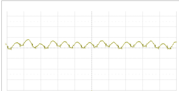
Output voltage ripple at: T_{P1} = +25^{\circ}\text{C} , V_i = 110\text{ V} , I_o = 2\text{ A} resistive load. Trace: output voltage (20 mV/div.). Time scale: (5 \mu\text{s} /div.). 20MHz bandwidth
