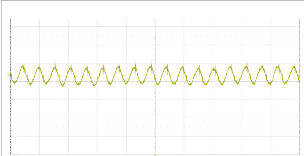
Output voltage ripple at: T_{P1} = +25^{\circ}\text{C} , V_i = 110\text{ V} , I_o = 2.5\text{ A} resistive load. Trace: output voltage (10 mV/div.). Time scale: (5 μs/div.). 20MHz bandwidth
