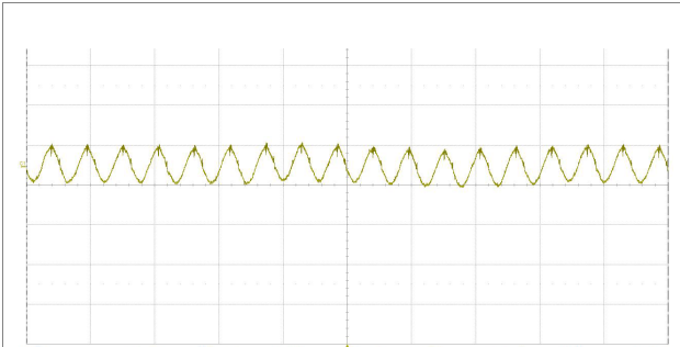
Output voltage ripple at: T_{P1} = +25^{\circ}\text{C} , V_i = 110\text{ V} , I_o = 1.25\text{ A} resistive load. Trace: output voltage (20 mV/div.), Time scale: (5 \mu\text{s} /div.), 20MHz bandwidth
