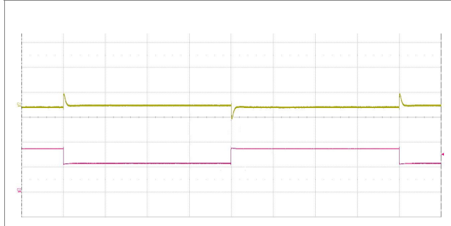
Output voltage response to load current step- change (1.25-1.875-1.25 A) at: T_{P1} = +25^{\circ}\text{C} , V_i = 110\text{ V} . Top trace: output voltage (200 mV/div.). Bottom trace: load current (1 A/div.). Time scale: (2 ms/div.).
