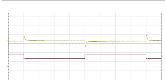
Output voltage response to load current step- change (1.0-1.5-1.0 A) at: T_{P1} = +25^{\circ}\text{C} , V_i = 110\text{ V} . Top trace: output voltage (500 mV/div.). Bottom trace: load current (1 A/div.). Time scale: (2 ms/div.).
