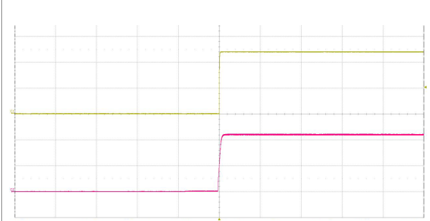
Start-up enabled by connecting V_i at: T_{P1} = +25^{\circ}\text{C} , V_i = 110\text{ V} , I_o = 2.5\text{ A} resistive load. Top trace: output voltage (5 V/div.). Bottom trace: input voltage (50 V/div.). Time scale: (200 ms/div.).
