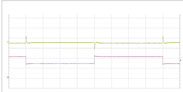
Output voltage response to load current step- change (3.0-4.5-3.0 A) at: T_{P1} = +25^{\circ}\text{C} , V_I = 110\text{ V} . Top trace: output voltage (100 mV/div.). Bottom trace: load current (2 A/div.). Time scale: (2 ms/div.).
