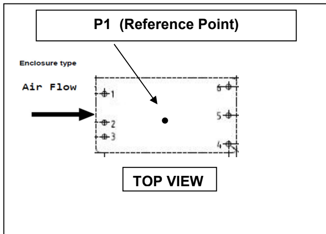
Reference point on PKE73XXA variant
