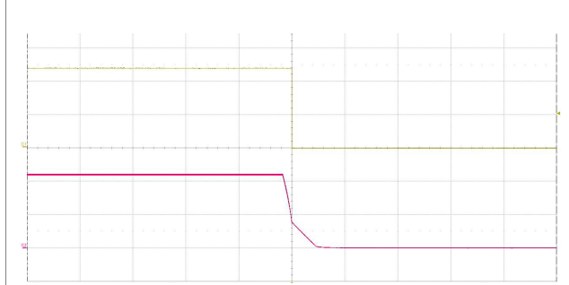
Start-up enabled by connecting V_i at: T_{P1} = +25^{\circ}\text{C} , V_i = 110\text{ V} , I_o = 2.5\text{ A} resistive load. Top trace: output voltage (5 V/div.). Bottom trace: input voltage (50 V/div.). Time scale: (200 ms/div.).
