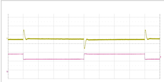
Output voltage response to load current step-change (0.625-0.937-0.625 A) at: T_{P1} = +25^{\circ}\text{C} , V_i = 110\text{ V} . Top trace: output voltage (200 mV/div.), Bottom trace: load current (500 mA/div.). Time scale: (2 ms/div.).
