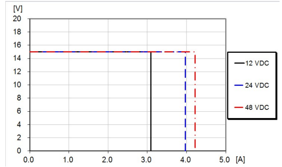
Output voltage vs. load current at I_o > \text{max } I_o at +25°C.
