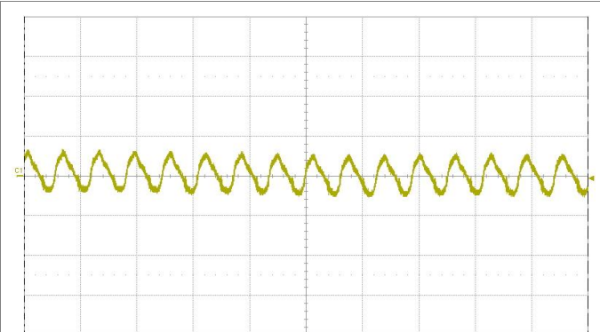
Output voltage ripple at: T_{P1} = +25^{\circ}\text{C} , V_i = 110\text{ V} , I_o = 3.8\text{ A} resistive load. Trace: output voltage (50 mV/div.). Time scale: (2 μs/div.). 20 MHz bandwidth.
