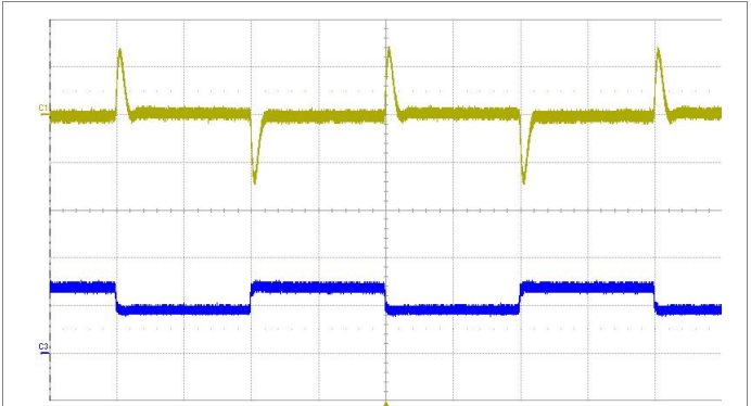
Output voltage response to load current step-change (1.9-2.85-1.9 A) at: T_{P1} = +25^{\circ}\text{C} , V_i = 110\text{ V} . Top trace: output voltage (500 mV/div.). Bottom trace: load current (2 A/div.). Time scale: (1 ms/div.).
