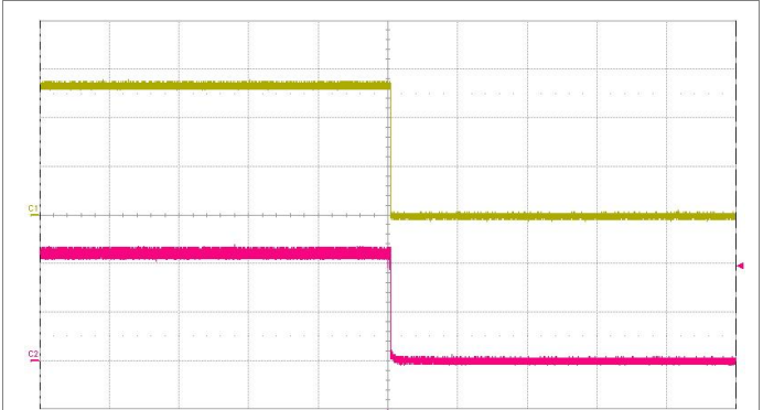
Shut-down enabled by disconnecting V_i at: T_{P1} = +25^{\circ}\text{C} , V_i = 110\text{ V} , I_o = 3.8\text{ A} resistive load. Top trace: output voltage (20 V/div.). Bottom trace: input voltage (50 V/div.). Time scale: (5 ms/div.).
