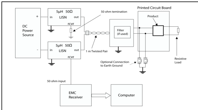
Test set-up
