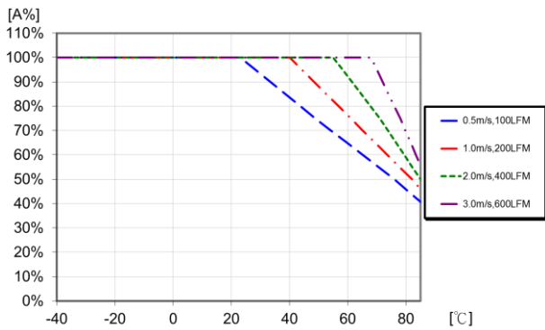
Available load current vs. ambient air temperature and airflow at V_1 = 110 V. See Thermal Consideration section.
