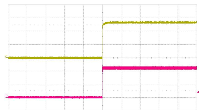
Start-up enabled by connecting V_i at: T_{P1} = +25^{\circ}\text{C} , V_i = 110\text{ V} , I_o = 3.8\text{ A} resistive load. Top trace: output voltage (20 V/div.). Bottom trace: input voltage (50 V/div.). Time scale: (10 ms/div.).
