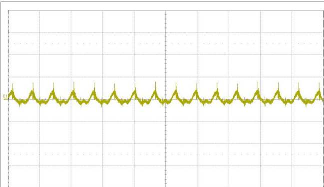
Output voltage ripple at: T_{P1} = +25^{\circ}\text{C} , V_I = 110\text{ V} , I_O = 8.4\text{ A} resistive load. Trace: output voltage (50 mV/div.). Time scale: (5 \mu\text{s} /div.). 20 MHz bandwidth.
