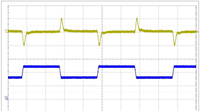
Output voltage response to load current step-change (8.4-12.6-8.4 A) at: T_{P1} = +25^{\circ}\text{C} , V_I = 110\text{ V} . Top trace: output voltage (500 mV/div.). Bottom trace: load current (5 A/div.). Time scale: (500 \mu\text{s} /div.).
