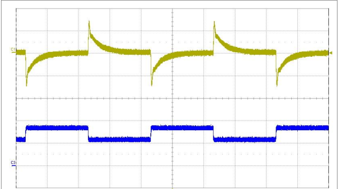
Output voltage response to load current step-change (2.1-3.15-2.1 A) at: T_{P1} = +25^{\circ}\text{C} , V_I = 110\text{ V} . Top trace: output voltage (500 mV/div.). Bottom trace: load current (2 A/div.). Time scale: (500 \mu\text{s} /div.).
