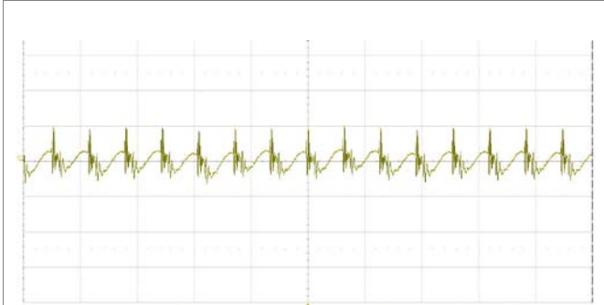
Output voltage ripple at: T_{P1} = +25^{\circ}\text{C} , V_i = 110\text{ V} , I_o = 13.33\text{ A} resistive load. Trace: output voltage (20 mV/div.). Time scale: (5 \mu\text{s} /div.). 20 MHz bandwidth
