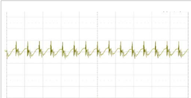
Output voltage ripple at: T_{P1} = +25^\circ\text{C} , V_i = 110\text{ V} , I_o = 14.5\text{ A} resistive load. Trace: output voltage (20 mV/div.). Time scale: (5 μs/div.). 20 MHz bandwidth
