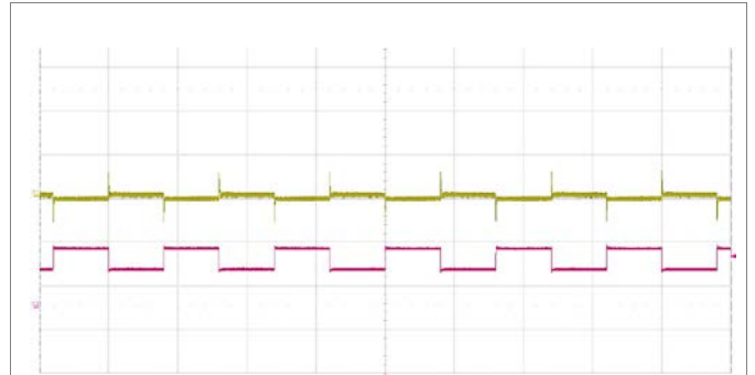
Output voltage response to load current step-change (7.25-10.87-7.25 A) at: T_{P1} = +25^\circ\text{C} , V_i = 110\text{ V} . Top trace: output voltage (500 mV/div.). Bottom trace: load current (5 A/div.). Time scale: (2 ms/div.).
