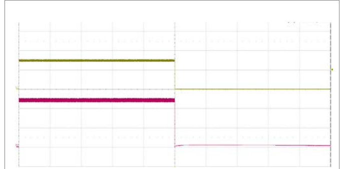
Shut-down enabled by disconnecting V_i at: T_{P1} = +25^{\circ}\text{C} , V_i = 110\text{ V} , I_o = 13.33\text{ A} resistive load. Top trace: output voltage (10 V/div.). Bottom trace: input voltage (50 V/div.). Time scale: (200 ms/div.).
