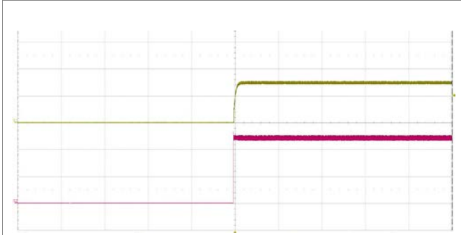
Start-up enabled by connecting V_i at: T_{P1} = +25^{\circ}\text{C} , V_i = 110\text{ V} , I_o = 13.33\text{ A} resistive load. Top trace: output voltage (10 V/div.). Bottom trace: input voltage (50 V/div.). Time scale: (200 ms/div.).
