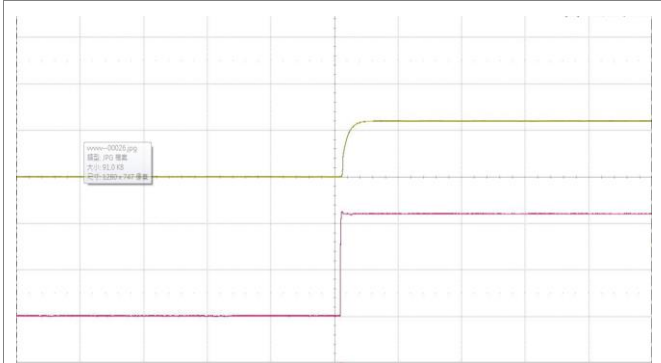
Start-up enabled by connecting V_i at: T_{P1} = +25\text{ }^\circ\text{C} , V_i = 110\text{ V} , I_o = 25\text{ A} resistive load. Top trace: output voltage (10 V/div.). Bottom trace: input voltage (50 V/div.). Time scale: (100 ms/div.).
