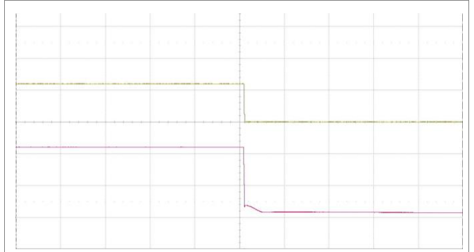
Shut-down enabled by disconnecting V_i at: T_{P1} = +25\text{ }^\circ\text{C} , V_i = 110\text{ V} , I_o = 25\text{ A} resistive load. Top trace: output voltage (10 V/div.). Bottom trace: input voltage (50 V/div.). Time scale: (100 ms/div.).
