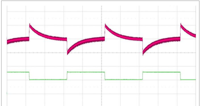
Output voltage response to load current step-change (10.85-16.275-10.85 A) at: T_{P1} = +25\text{ }^\circ\text{C} , V_I = 110\text{ V} . Top trace: output voltage (100 mV/div.). Bottom trace: load current (10 A/div.). Time scale: (10 ms/div.).
