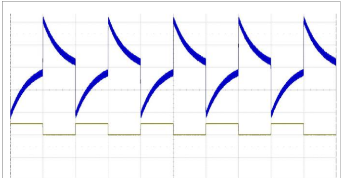
Output voltage response to load current step-change (10-15-10 A) at: T_{P1} = +25\text{ }^\circ\text{C} , V_I = 110\text{ V} . Top trace: output voltage (50 mV/div.). Bottom trace: load current (10 A/div.). Time scale: (10 ms/div.).
