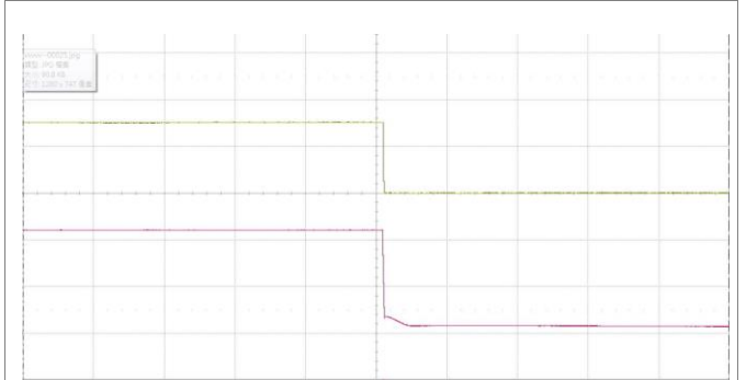
Shut-down enabled by disconnecting V_I at: T_{P1} = +25\text{ }^\circ\text{C} , V_I = 110\text{ V} , I_O = 20\text{ A} resistive load. Top trace: output voltage (10 V/div.). Bottom trace: input voltage (50 V/div.). Time scale: (100 ms/div.).
