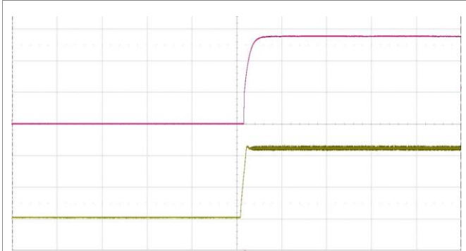
Start-up enabled by connecting V_I at: T_{P1} = +25\text{ }^\circ\text{C} , V_I = 110\text{ V} , I_O = 21.7\text{ A} resistive load. Top trace: output voltage (5 V/div.). Bottom trace: input voltage (50 V/div.). Time scale: (100 ms/div.).
