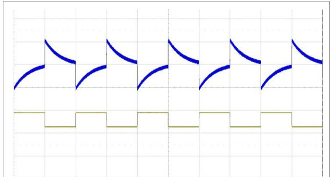
Output voltage response to load current step-change (12.5-18.75-12.5 A) at: T_{P1} = +25\text{ }^\circ\text{C} , V_i = 110\text{ V} . Top trace: output voltage (100 mV/div.). Bottom trace: load current (10 A/div.). Time scale: (10 ms/div.).
