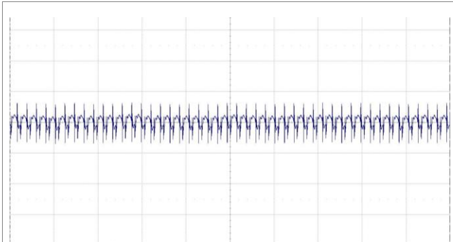
Output voltage ripple at: T_{P1} = +25\text{ }^\circ\text{C} , V_I = 110\text{ V} , I_O = 20\text{ A} resistive load. Trace: output voltage (50 mV/div.). Time scale: (20 μs/div.). 20 MHz bandwidth.
