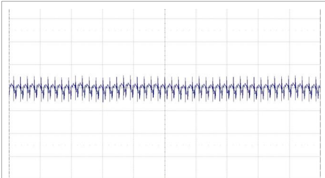
Output voltage ripple at: T_{P1} = +25\text{ }^\circ\text{C} , V_i = 110\text{ V} , I_o = 25\text{ A} resistive load. Trace: output voltage (50 mV/div.). Time scale: (20 \mu\text{s} /div.). 20 MHz bandwidth.
