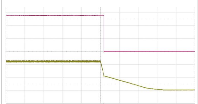
Shut-down enabled by disconnecting V_I at: T_{P1} = +25\text{ }^\circ\text{C} , V_I = 110\text{ V} , I_O = 21.7\text{ A} resistive load. Top trace: output voltage (5 V/div.). Bottom trace: input voltage (50 V/div.). Time scale: (100 ms/div.).
