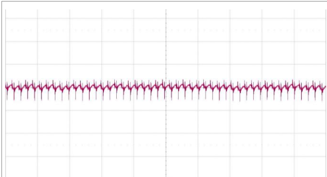
Output voltage ripple at: T_{P1} = +25\text{ }^\circ\text{C} , V_I = 110\text{ V} , I_O = 21.7\text{ A} resistive load. Trace: output voltage (50 mV/div.). Time scale: (20 \mu\text{s} /div.). 20 MHz bandwidth.
