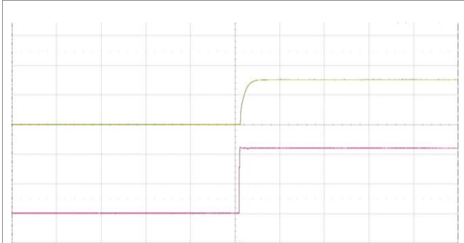
Start-up enabled by connecting V_I at: T_{P1} = +25\text{ }^\circ\text{C} , V_I = 110\text{ V} , I_O = 20\text{ A} resistive load. Top trace: output voltage (10 V/div.). Bottom trace: input voltage (50 V/div.). Time scale: (100 ms/div.).
