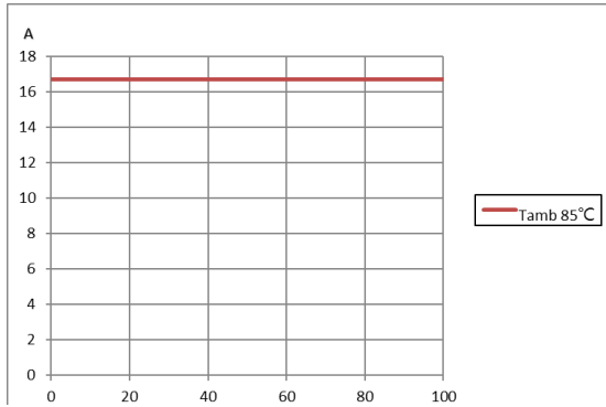
Available load current vs. cold wall temperature. V_1 = 36\text{ V} . See Thermal Consideration section.
