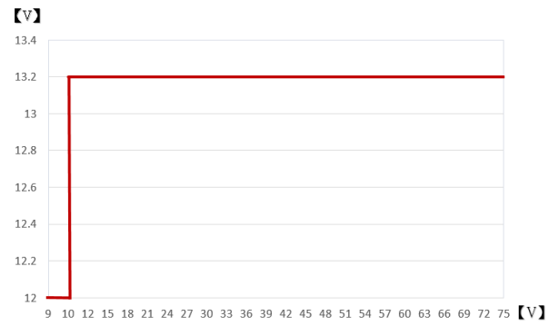
Max adjustable output voltage vs. input voltage at TP_1 = +25\text{ °C} . Max adjustable output voltage \geq 12\text{ V} at V_1 = 9\text{ V} , P_o = 200\text{ W}
