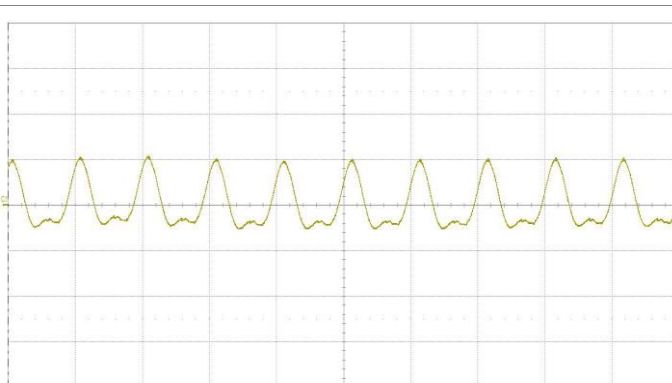
Output voltage ripple at: T_{P1} = +25^\circ\text{C} , V_I = 36\text{ V} , I_O = 4.2\text{ A} resistive load. Trace: output voltage (100 mV/div.), Time scale: (5 \mu\text{s} /div.), 20 MHz bandwidth.
