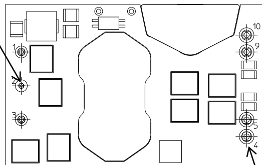
Pin 4 for measurement of minimum pin (solder joint) temperature, T_{PIN}
