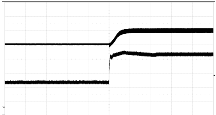
HRR product output at input voltage step 36-75 V, 1 ms/div Bottom trace – input voltage change 36-75 V, 20 V/div Top trace – resulting output voltage change, 1 V/div
