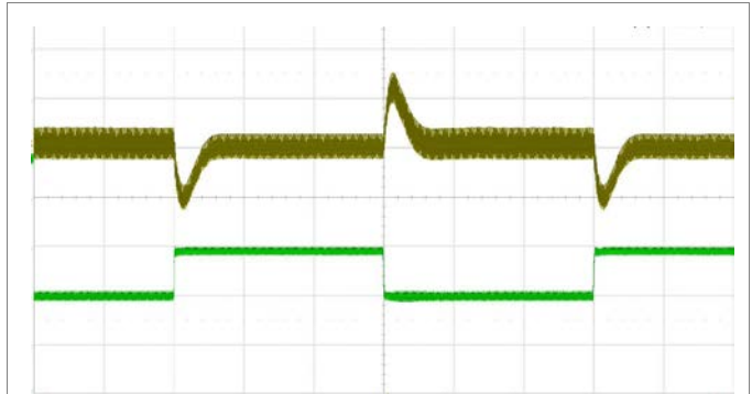
Output voltage response to load current step-change (1.80-2.70-1.80 A) at: T_{P1} = +25^{\circ}\text{C} , V_i = 72\text{ V} .
