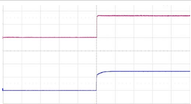
Start-up enabled by connecting V_I at: T_{P1} = +25^\circ\text{C} , V_I = 72\text{ V} , I_O = 15.2\text{ A} resistive load. Top trace: output voltage (2 V/div.). Bottom trace: input voltage (50 V/div.). Time scale: (50 ms/div.).
