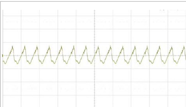
Output voltage ripple at: T_{P1} = +25^{\circ}\text{C} , V_I = 72\text{ V} , I_O = 0.95\text{ A} resistive load. Trace: output voltage (200 mV/div.). Time scale: (10 \mu\text{s} /div.). 20 MHz bandwidth.
