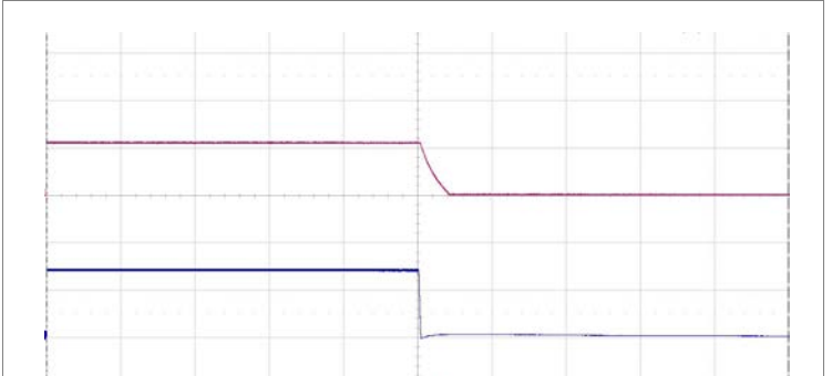
Shut-down enabled by disconnecting V_I at: T_{P1} = +25^\circ\text{C} , V_I = 72\text{ V} , I_O = 0.95\text{ A} resistive load. Top trace: output voltage (50 V/div.). Bottom trace: input voltage (50 V/div.). Time scale: (5 ms/div.).
