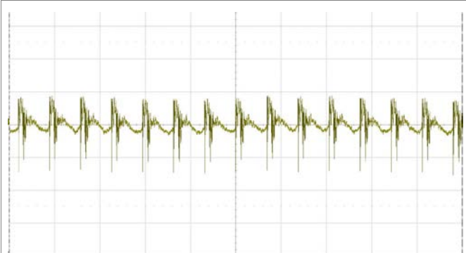
Output voltage ripple at: T_{P1} = +25^{\circ}\text{C} , V_I = 72\text{ V} , I_O = 15.2\text{ A} resistive load. Trace: output voltage (20 mV/div.). Time scale: (10 \mu\text{s} /div.). 20 MHz bandwidth.
