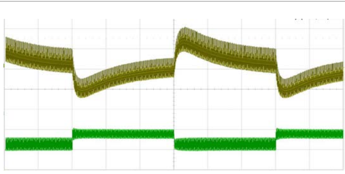
Output voltage response to load current step-change (0.525-0.7875-0.525 A) at: T_{P1} = +25^{\circ}\text{C} , V_I = 72\text{ V} . Top trace: output voltage (200mV/div.). Bottom trace: load current (500m A/div.). Time scale: (500 μs/div.).
