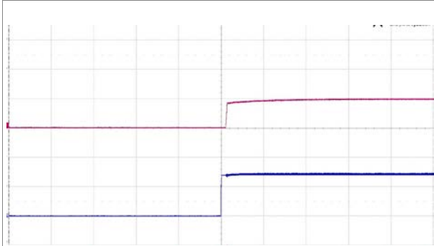
Start-up enabled by connecting V_I at: T_{P1} = +25^{\circ}\text{C} , V_I = 72\text{ V} , I_O = 1.05\text{ A} resistive load. Top trace: output voltage (50 V/div.). Bottom trace: input voltage (50 V/div.). Time scale: (50 ms/div.).
