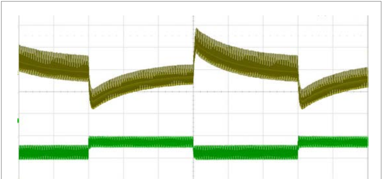
Output voltage response to load current step-change (0.475-0.7125-0.475 A) at: T_{P1} = +25^\circ\text{C} , V_I = 72\text{ V} . Top trace: output voltage (200mV/div.). Bottom trace: load current (500 mA/div.). Time scale: (500 μs/div.).
