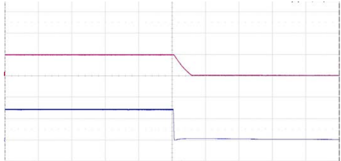
Shut-down enabled by disconnecting V_I at: T_{P1} = +25^{\circ}\text{C} , V_I = 110\text{ V} , I_O = 1.05\text{ A} resistive load. Top trace: output voltage (50 V/div.). Bottom trace: input voltage (50 V/div.). Time scale: (5 ms/div.).
