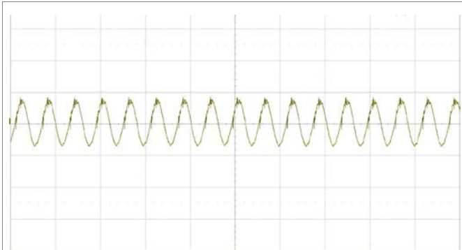
Output voltage ripple at: T_{P1} = +25^{\circ}\text{C} , V_i = 72\text{ V} , I_o = 3.60\text{ A} resistive load.
