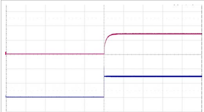
Start-up enabled by connecting V_i at: T_{P1} = +25^{\circ}\text{C} , V_i = 72\text{ V} , I_o = 3.60\text{ A} resistive load.
