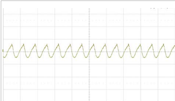
Output voltage ripple at: T_{P1} = +25^{\circ}\text{C} , V_I = 72\text{ V} , I_O = 1.05\text{ A} resistive load. Trace: output voltage (200 mV/div.). Time scale: (10 μs/div.). 20 MHz bandwidth.
