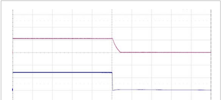
Shut-down enabled by disconnecting V_I at: T_{P1} = +25^{\circ}\text{C} , V_I = 72\text{ V} , I_O = 0.95\text{ A} resistive load. Top trace: output voltage (50 V/div.). Bottom trace: input voltage (50 V/div.). Time scale: (5 ms/div.).
