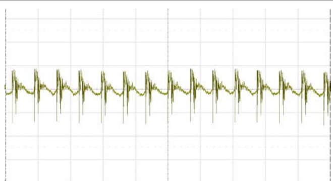
Output voltage ripple at: T_{P1} = +25^\circ\text{C} , V_I = 72\text{ V} , I_O = 15.2\text{ A} resistive load. Trace: output voltage (20 mV/div.). Time scale: (10 μs/div.). 20 MHz bandwidth.
