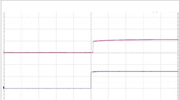
Start-up enabled by connecting V_I at: T_{P1} = +25^\circ\text{C} , V_I = 72\text{ V} , I_O = 0.95\text{ A} resistive load. Top trace: output voltage (50 V/div.). Bottom trace: input voltage (50 V/div.). Time scale: (50 ms/div.).
