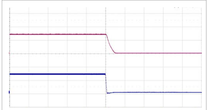
Shut-down enabled by disconnecting V_i at: T_{P1} = +25^{\circ}\text{C} , V_i = 72\text{ V} , I_o = 3.60\text{ A} resistive load.
