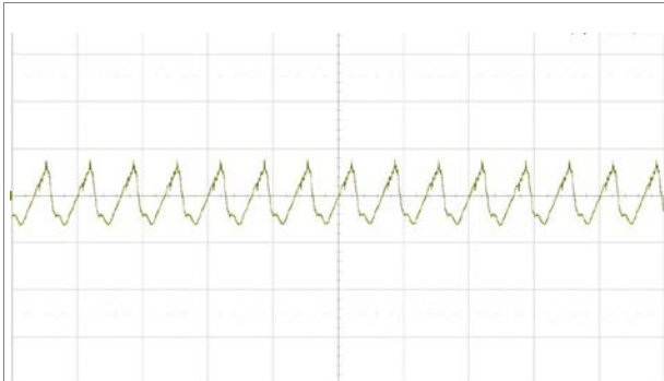
Output voltage ripple at: T_{P1} = +25^\circ\text{C} , V_I = 72\text{ V} , I_O = 0.95\text{ A} resistive load. Trace: output voltage (200 mV/div.). Time scale: (10 μs/div.). 20 MHz bandwidth.
