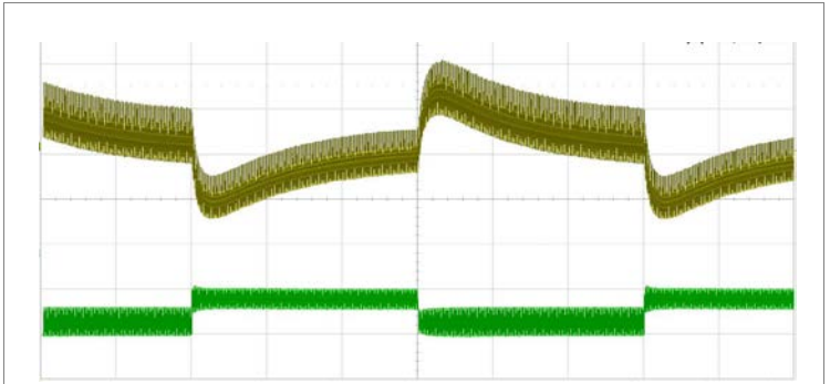
Output voltage response to load current step-change (0.525-0.7875-0.525 A) at: T_{P1} = +25^{\circ}\text{C} , V_I = 72\text{ V} . Top trace: output voltage (200mV/div). Bottom trace: load current (500m A/div). Time scale: (500 μs/div.).
