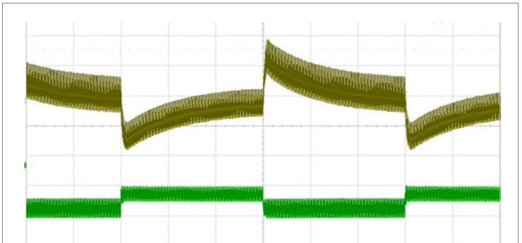
Output voltage response to load current step-change (0.475-0.7125-0.475 A) at: T_{P1} = +25^{\circ}\text{C} , V_I = 72\text{ V} . Top trace: output voltage (200mV/div.). Bottom trace: load current (500 mA/div.). Time scale: (500 \mu\text{s} /div.).
