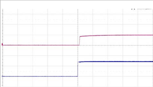
Start-up enabled by connecting V_I at: T_{P1} = +25^{\circ}\text{C} , V_I = 72\text{ V} , I_O = 1.05\text{ A} resistive load. Top trace: output voltage (50 V/div). Bottom trace: input voltage (50 V/div). Time scale: (50 ms/div.).
