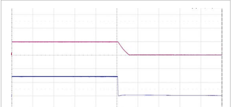
Shut-down enabled by disconnecting V_I at: T_{P1} = +25^{\circ}\text{C} , V_I = 110\text{ V} , I_O = 1.05\text{ A} resistive load. Top trace: output voltage (50 V/div). Bottom trace: input voltage (50 V/div). Time scale: (5 ms/div.).
