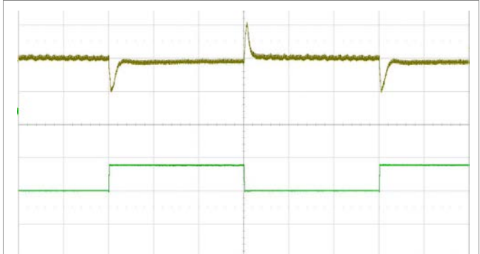
Output voltage response to load current step-change (7.6-11.4-7.6 A) at: T_{P1} = +25^\circ\text{C} , V_I = 72\text{ V} . Top trace: output voltage (100 mV/div.). Bottom trace: load current (5 A/div.). Time scale: (500 μs/div.).
