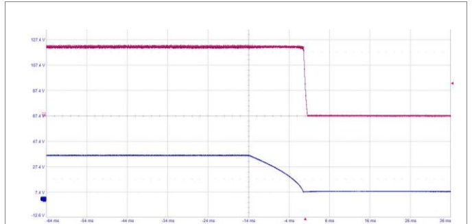
Shut-down enabled by disconnecting V I at: T P1 = +25°C, V I = 36 V, I O = 1.85 A resistive load. Top trace: output voltage (20 V/div.). Bottom trace: input voltage (20 V/div.). Time scale: (10 ms/div.).
