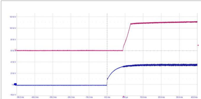
Start-up enabled by connecting V I at: T P1 = +25°C, V I = 36 V, I O = 1.85 A resistive load. Top trace: output voltage (20 V/div.). Bottom trace: input voltage (20 V/div.). Time scale: (10 ms/div.).
