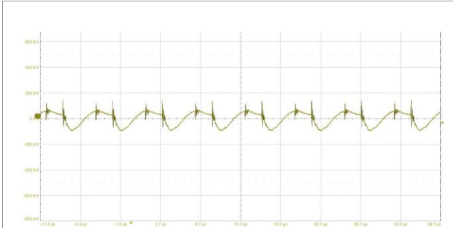
Output voltage ripple at: T P1 = +25°C, V I = 36 V, I O = 1.85 A resistive load. Trace: output voltage (200 mV/div.). Time scale: (5 μs/div.). 20 MHz bandwidth.
