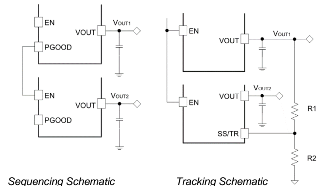
Sequencing Schematic
