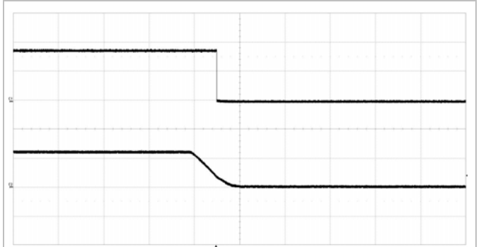
Shut-down enabled by disconnecting V_I at: T_{P1} = +25^{\circ}\text{C} , V_I = 24\text{ V} , I_O = 6\text{ A} resistive load. Top trace: output voltage 1 V/div. Bottom trace: input voltage 20 V/div. Time scale: 50 ms/div.
