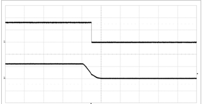
Shut-down enabled by disconnecting V_I at: T_{P1} = +25^{\circ}\text{C} , V_I = 24\text{ V} , I_O = 6\text{ A} resistive load. Top trace: output voltage 2 V/div. Bottom trace: input voltage 20 V/div. Time scale: 50 ms/div.
