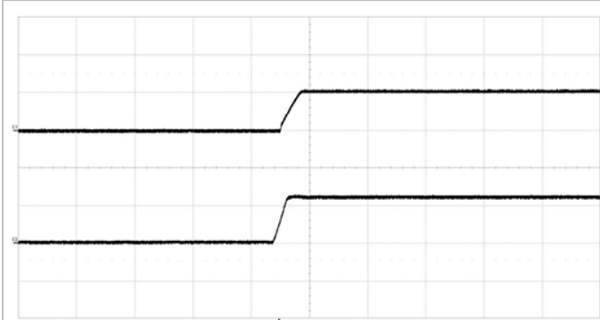
Start-up enabled by connecting V_I at: T_{P1} = +25^{\circ}\text{C} , V_I = 24\text{ V} , I_O = 6\text{ A} resistive load. Top trace: output voltage 5 V/div. Bottom trace: input voltage 20 V/div. Time scale: 10 ms/div.
