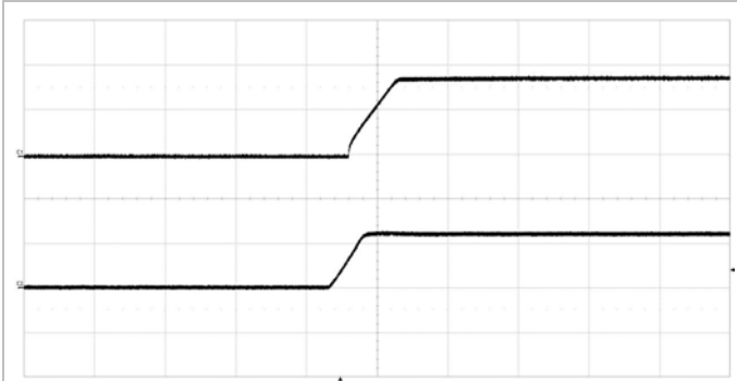
Start-up enabled by connecting V_I at: T_{P1} = +25^{\circ}\text{C} , V_I = 24\text{ V} , I_O = 6\text{ A} resistive load. Top trace: output voltage 1 V/div. Bottom trace: input voltage 20 V/div. Time scale: 5 ms/div.
