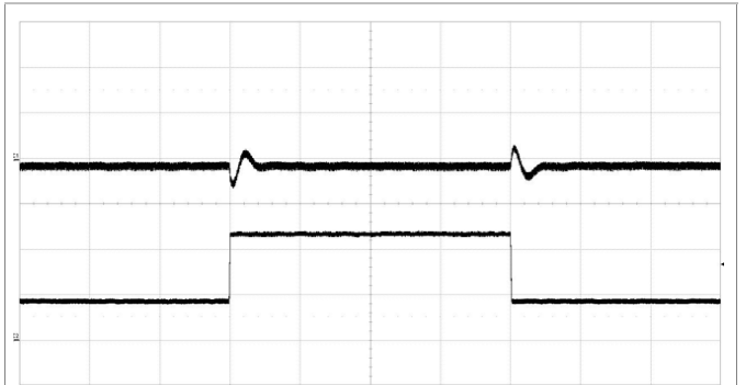
Output voltage response to load current step- change 1.5-4.5-1.5 A at: T_{P1} = +25^{\circ}\text{C} , V_I = 24\text{ V} . C_{OUT} = 2 \times 47\text{ }\mu\text{F Ceramic} + 330\text{ }\mu\text{F Polymer} Top trace: output voltage 100 mV/div. Bottom trace: load current 2 A/div. Time scale: 200 \mu\text{s} /div. Slew rate: 1A/ \mu\text{s} . 20 MHz bandwidth.
