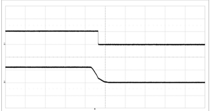
Shut-down enabled by disconnecting V_I at: T_{P1} = +25^{\circ}\text{C} , V_I = 24\text{ V} , I_O = 6\text{ A} resistive load. Top trace: output voltage 5 V/div. Bottom trace: input voltage 20 V/div. Time scale: 50 ms/div.
