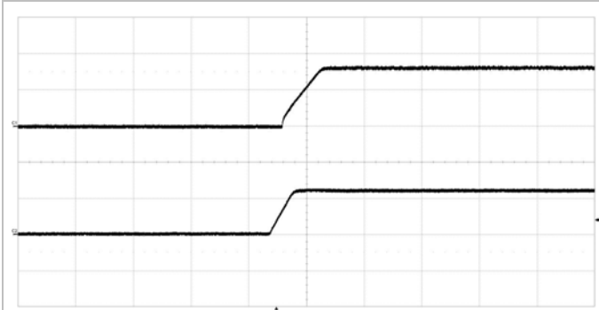
Start-up enabled by connecting V_I at: T_{P1} = +25^{\circ}\text{C} , V_I = 24\text{ V} , I_O = 6\text{ A} resistive load. Top trace: output voltage 2 V/div. Bottom trace: input voltage 20 V/div. Time scale: 50 ms/div.
