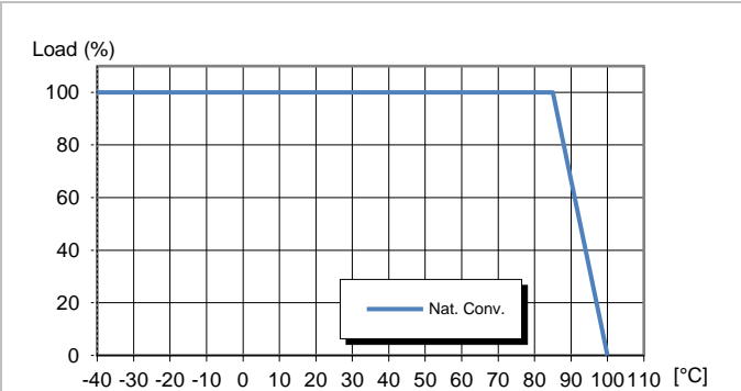
PUA03-1A, PUA05-1A, PUA12-1A Available load vs. ambient air temperature. See Thermal Consideration section.
