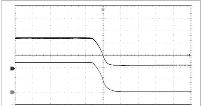
Shut-down, closed by disconnecting V_I at: T_{P1} = +25^\circ\text{C} , V_I = 5\text{ V} , V_O = 5\text{ V} I_O = 200\text{ mA} resistive load.
