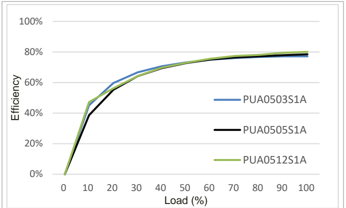
PUA05-1A Efficiency vs. load current at T_{P1} = +25^{\circ}\text{C} .
