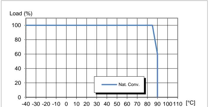
PUA24-1A Available load vs. ambient air temperature. See Thermal Consideration section.
