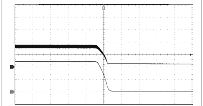
Shut-down, closed by disconnecting V_I at: T_{P1} = +25^\circ\text{C} , V_I = 3.3\text{ V} , V_O = 5\text{ V} I_O = 200\text{ mA} resistive load.
