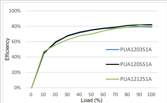
PUA12-1A Efficiency vs. load current at T_{P1} = +25^{\circ}\text{C} .
