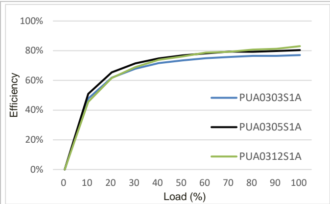
PUA03-1A Efficiency vs. load current at T_{P1} = +25^{\circ}\text{C} .
