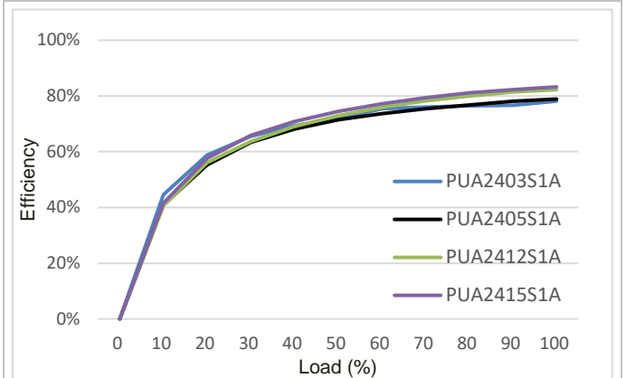
PUA24-1A Efficiency vs. load current at T_{P1} = +25^{\circ}\text{C} .
