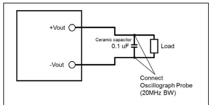
Output ripple and noise test setup
