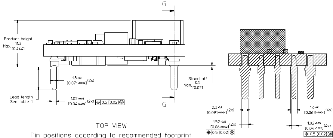
Section G-G
